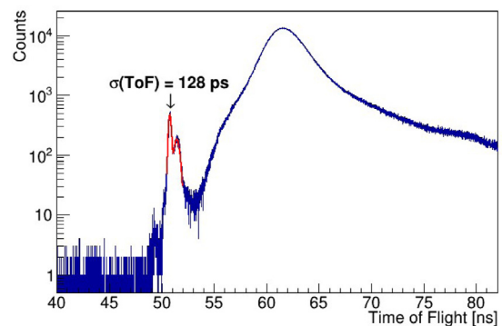
Fig. 17. ToF distribution measured between the start counter and NeuLAND for ^{120}\text{Sn} on a Pb-target at 800 MeV/nucleon, corrected for the difference in flight path for gamma-rays to the interaction position in NeuLAND.
