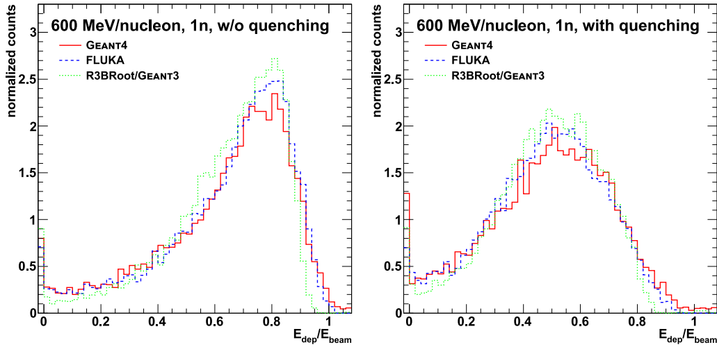
Fig. 3. Simulated distributions of deposited energy E_{\text{dep}} divided by incoming neutron energy E_{\text{beam}} = 600 \text{ MeV} . The neutrons hit the plastic detector volume of 250 \times 250 \times 300 \text{ cm}^3 at the central part. The graphics displays on the left hand side the distribution before light quenching correction, on the right hand side the distribution after light quenching correction. We compare simulations using GEANT4 (solid red curve), FLUKA (dashed blue curve), and GEANT3 (dotted green curve).
