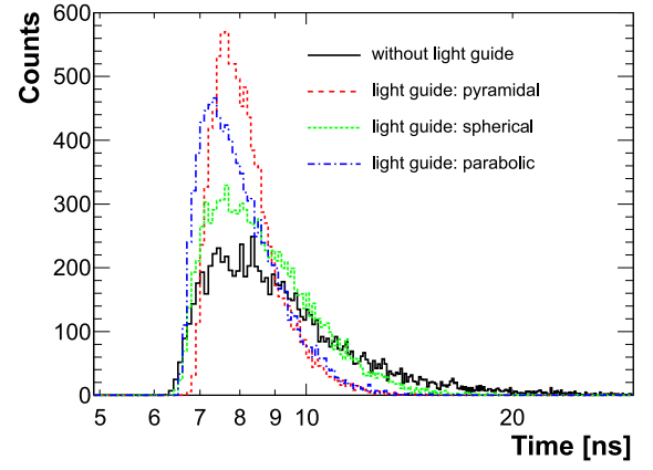
Fig. 5. Arrival time distributions of photons from simulations with different light guide shapes for an entrance window of a photomultiplier with a diameter of 1 inch.
