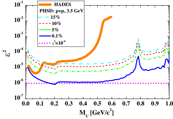
FIG. 5. The kinetic mixing parameter \epsilon^2 extracted from the PHSD dilepton spectra for p + p at 3.5 GeV calculated for different \epsilon^2 scenarios in comparison with the combined HADES results (orange line) [15] (as in Fig. 3). The PHSD results are shown with 0.1%, 5%, 10%, and 15% allowed surplus of the U -boson contributions over the total SM yield (cf. color coding in the legend). The dotted magenta line shows the constant \epsilon^2 = 10^{-6} .
