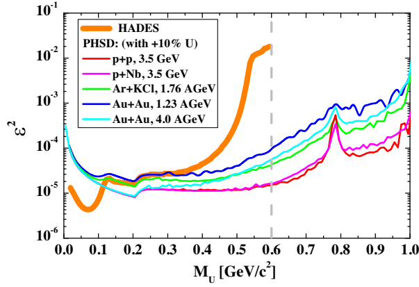
FIG. 3. The kinetic mixing parameter \epsilon^2 extracted from the PHSD dilepton spectra for p + p at 3.5 GeV (red line), p + \text{Nb} at 3.5 GeV (magenta line), \text{Ar} + \text{KCl} at 1.76 A GeV (green line), \text{Au} + \text{Au} at 1.23 A GeV (blue line), and \text{Au} + \text{Au} at 4.0 A GeV in comparison with the combined HADES results (orange line) [15]. The PHSD results are shown with 10% allowed surplus of the U -boson contributions over the total SM yield, i.e., C_U = 0.1 .
