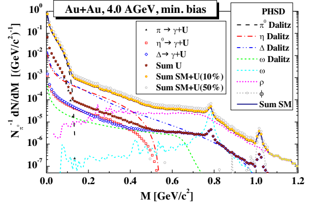
FIG. 2. The PHSD predictions for the mass differential dilepton spectra dN/dM —normalized to the \pi^0 multiplicity—for minimum bias Au + Au collisions at 4.0 A GeV. The color coding of the individual lines is the same as in Fig. 1. The contributions from U \rightarrow e^+e^- are shown with 10% allowed surplus of total SM yield. Additionally, the gray open dots show the sum of all SM and U -boson contributions with 50% allowed surplus of the total SM yield.
