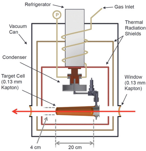
Figure 31. The cryotarget at HI \gamma S [206].
