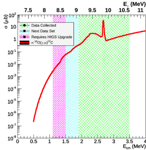
Figure 10. Plot of the cross section of the ^{16}\text{O}(\gamma, \alpha)^{12}\text{C} reaction as a function the system center-of-mass energy (bottom axis) and the incident \gamma -ray beam energy (top axis). The green hash shows the region where data have been collected at HI \gamma S using the optical time-projection chamber (TPC). The blue filled bar is the lowest energy region experimentally accessible at HI \gamma S using current target and detector technologies. The energy region indicated by the red brick filled area is what would be possible with an intensity upgrade of HI \gamma S.
