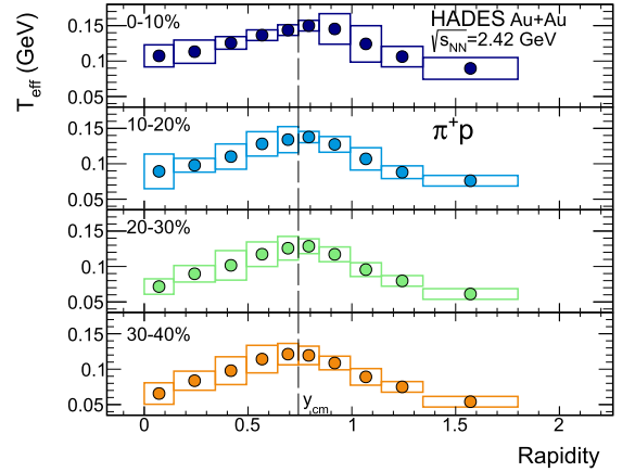
Fig. 7. Effective temperature T_{eff} obtained from fits of Eq. (2) to the transverse momentum distribution of \pi^+p pairs with invariant masses between 1.1 and 1.4 GeV/c 2 . The long-dashed line shows the center-of-mass rapidity y_{cm} = 0.74 .
