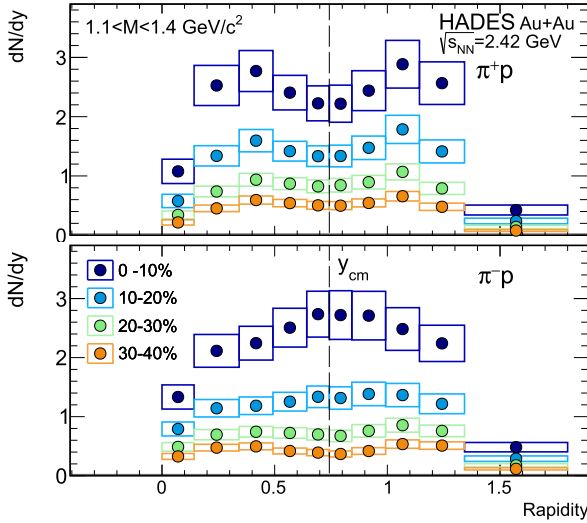
Fig. 8. Rapidity density distributions of correlated \pi^+p (top panel) and \pi^-p (bottom panel) pairs integrated within the 1.1 < M_{\text{inv}} ( \text{GeV}/c^2 ) < 1.4 range for four centrality classes. The boxes represent the systematic errors of the measurement. The long-dashed lines represent the mid-rapidity.
