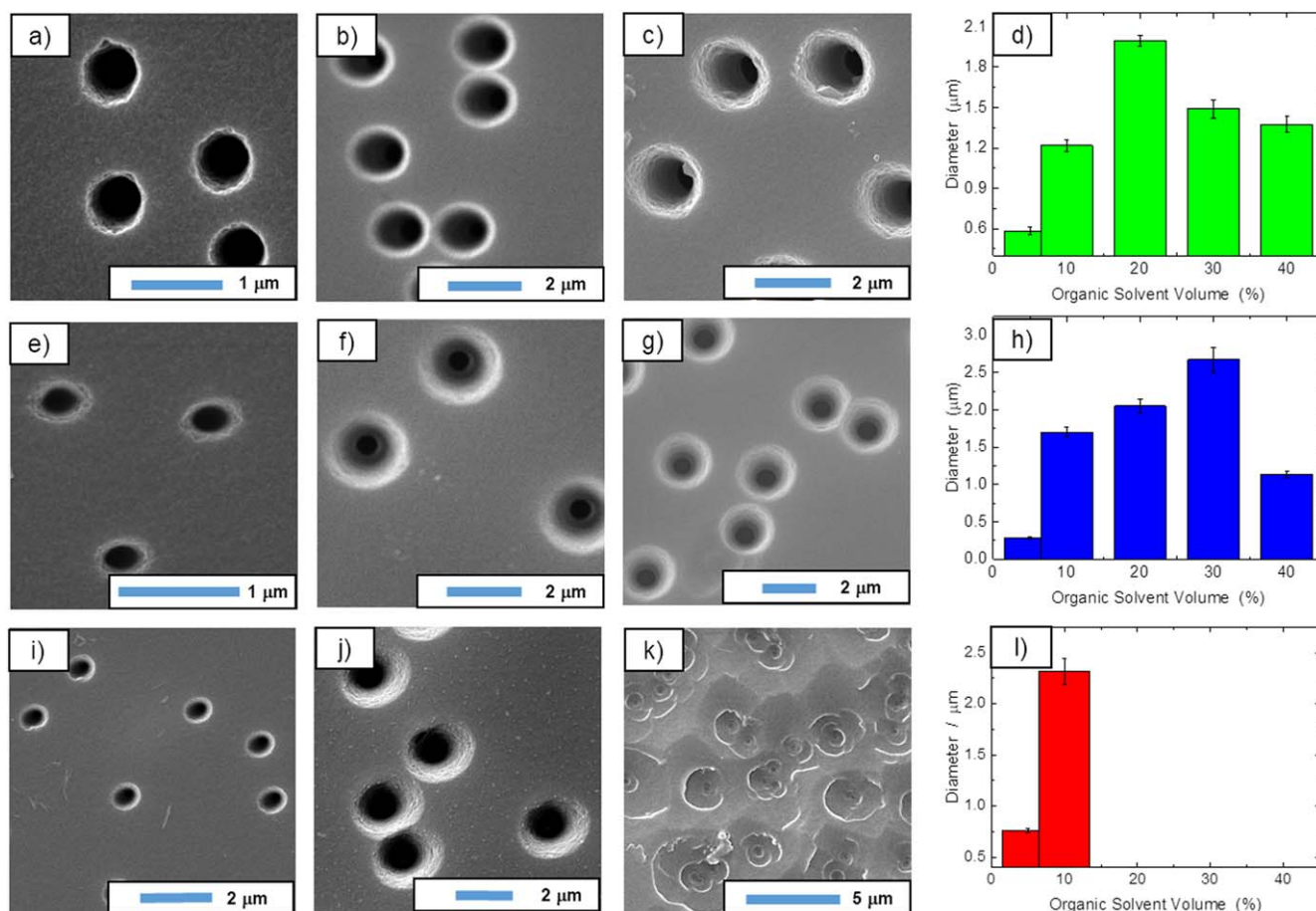
Figure 6. Solvent dependent symmetrical etching of PI membranes ( 10^7 pores \text{cm}^{-2} ) with mixtures of NaOCl/solvent at 50 °C. SEM images after 45 min etching with 5%, 10% and 20% of ACN (a)–(c), THF (e)–(g) and EtOH (i)–(k), and the effect of NaOCl/organic solvent on the pore diameter in case of ACN (d), THF (h) and EtOH (l).
