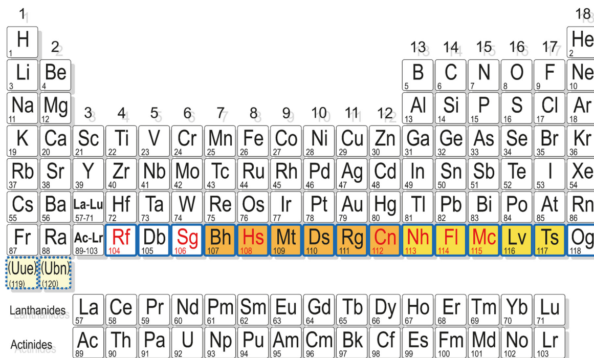
Figure 2: Periodic table of the elements. Superheavy elements are shown in blue-bordered boxes. Elements discovered at GSI are marked by orange-filled boxes, and those confirmed at GSI before their official approval by yellow-filled boxes. Elements with symbols given in red have been chemically studied at GSI; in several cases, these were the first chemical studies of these elements. Elements 119 and 120 have not yet been discovered.
