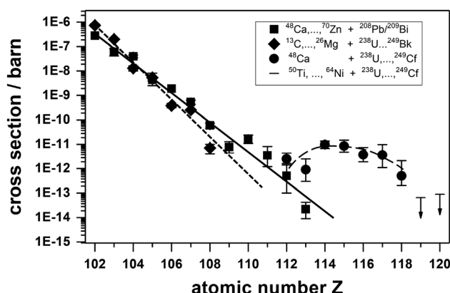
Figure 7: Experimentally measured maximum cross sections for the production of elements with Z = 102 – 118 as well as lowest reported upper limits for elements with Z = 119 and 120 . The fits (solid: Cold fusion reactions; short-dashed: Hot-fusion reactions with light projectiles; long-dashed: ^{48}\text{Ca} -induced reactions) are shown to guide the eye.
