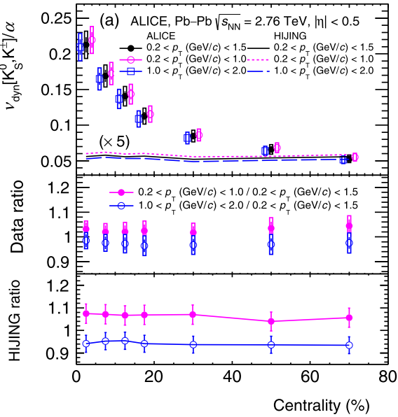
Fig. 4. (a) top: measured and HIJING (generator level) predicted values of v_{\text{dyn}}[K_S^0, K^\pm]/\alpha as a function of collision centrality for various transverse momentum interval of charged kaons. HIJING predicted scaled values are multiplied by a factor of 5 to approximately match the measured values in most peripheral collisions; middle: ratio of data for various transverse momentum interval as a function of centrality; bottom: ratio of HIJING for various transverse momentum interval as a function of centrality.
