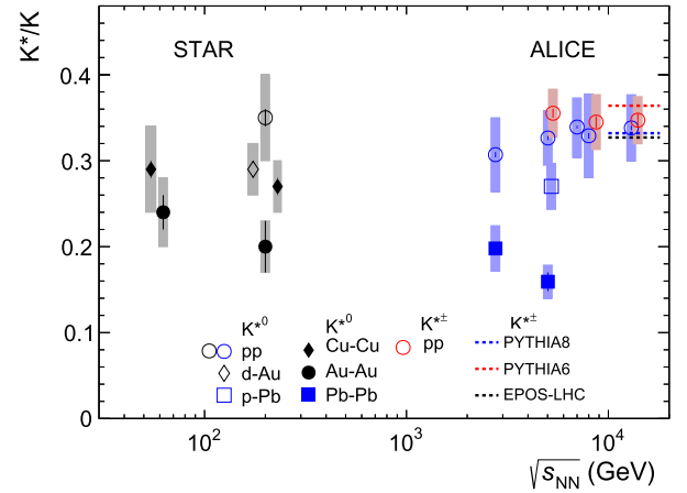
Fig. 6. Particle ratios K^{*\pm}/K and K^0/K , depicted as K^*/K , in pp [3,8–11,17,26,33–35], central d-Au [36], central p-Pb [12] and central A-A [8–10,35,37] collisions as a function of \sqrt{s_{\text{NN}}} . For the d-Au data, the numerator yield is derived from a combination of K^0 and K^{*\pm} states. Bars represent the statistical uncertainties and boxes represent the systematic uncertainties. The points for K^0 for d-Au, Cu-Cu and p-Pb collisions and for K^{*\pm} for pp collisions have been shifted horizontally for visibility. Red, blue and black lines represent the K^{*\pm}/K ratio predicted with PYTHIA6-Perugia 2011 [30], PYTHIA8-Monash 2013 [31] and EPOS-LHC [6], respectively.
