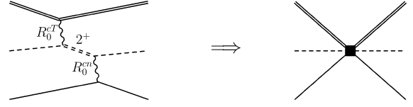
Fig. 1. Illustration of the effective three-body force that arises from the virtual excitation of the ^{10}\text{Be} core to the 2^+ state. At long wavelengths/low energies the mechanism shown in the left part of the figure can be replaced by the effective three-body force shown in the right part. R_0^{cT} and R_0^{cn} represent, respectively, the range of the core-target and core-neutron interactions.
