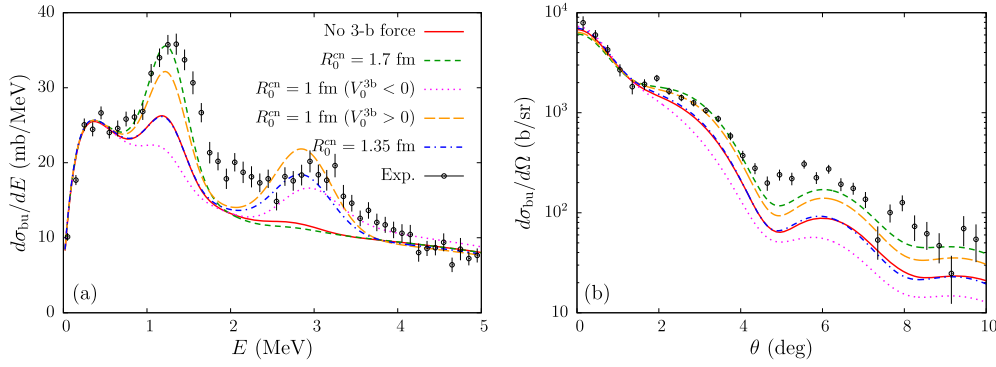
Fig. 3. Influence of the range of the three-body force (4) in the c - n relative coordinate R_0^{cn} in the breakup of ^{11}\text{Be} on ^{12}\text{C} at 67 MeV/nucleon. (a) Energy distribution; (b) angular distribution for the breakup at energies around the \frac{5}{2}^+ resonance. The range R_0^{cT} is kept to its 3.5 fm optimum. Experimental data from Ref. [6].
