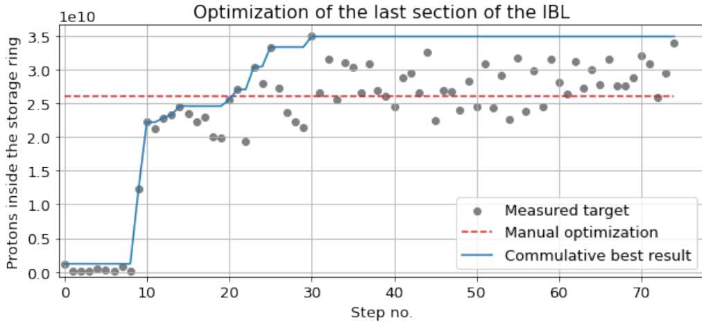
Figure 4. Optimizing the quadrupole and steering magnets of the last section from the IBL via Bayesian optimization. After manual optimization of the IBL there were 2.6 \times 10^{10} protons inside the synchrotron. The objective function for Bayesian optimization is the beam current inside COSY and the parameters space is of size d = 8 . The beam intensity after the optimization improved to 3.5 \times 10^{10} protons inside the synchrotron and the duration of this optimization was 19 minutes.
