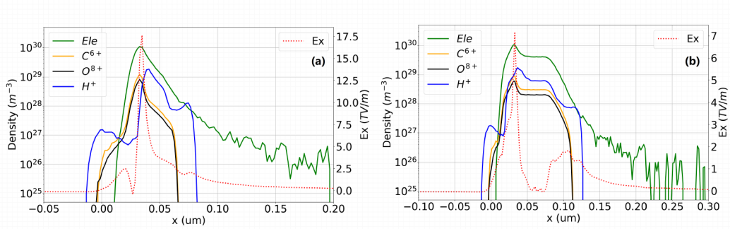
Fig. 5.7: When T = -20 fs, the leading edge of the main pulse reaches the target. When the laser drives the plasma, it compresses and accelerates all ions. For the 40 nm target (a), the proton beam is separated from the heavy ions during acceleration and modulates the accelerating electric field. However, for the 90 nm target (b), the protons and heavy ions mix together during acceleration.
