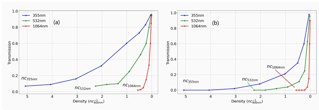
Fig. 6.5: Numerical calculation results of probe light transmittance as a function of peak plasma densities. The initial target is 90 nm. (a) The pre-pulse intensity is 5 \times 10^{13} \text{W/cm}^2 , and (b) The pre-pulse intensity is 3 \times 10^{15} \text{W/cm}^2 . The plasma density has been normalized by nC_{800nm} .
