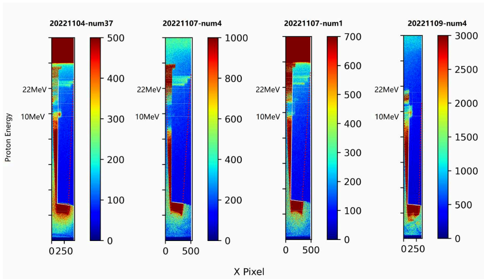
Fig. 1: The raw energy spectrum of circularly polarized light incident on the thin target. From the left to the right are 10 nm, 40 nm, 50 nm, and 90 nm thickness targets, respectively.
