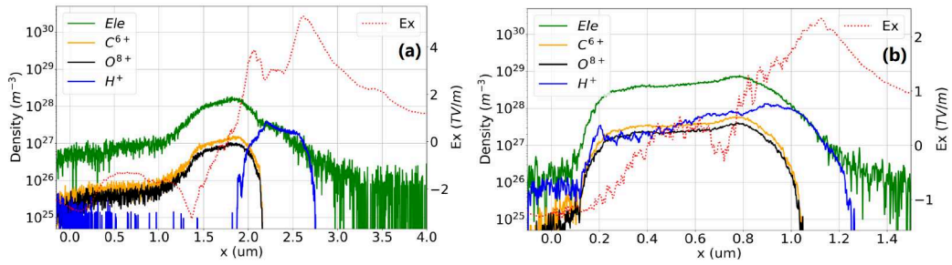
Fig. 5.9: Driving the laser light away from the interaction region ( T = 40.0 fs). (a) is the 40 nm target, and (b) is the 90 nm target. The Ex-field peak is dominated by the local electrons and ions.
