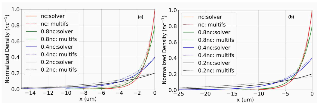
Fig. 6.3: Spatial distribution of plasmas with different maximum densities. Initial thickness is 90 nm, and the pre-pulse intensity is 5 \times 10^{13} \text{W/cm}^2 . (a) and (b) correspond to 355 nm and 532 nm probe light, and plasma densities are normalized by n_{c355\text{nm}} and n_{c532\text{nm}} , respectively. “multifs” means the multifs outputs the plasma density profile and “solver” means the plasma density profile used in the solver.
