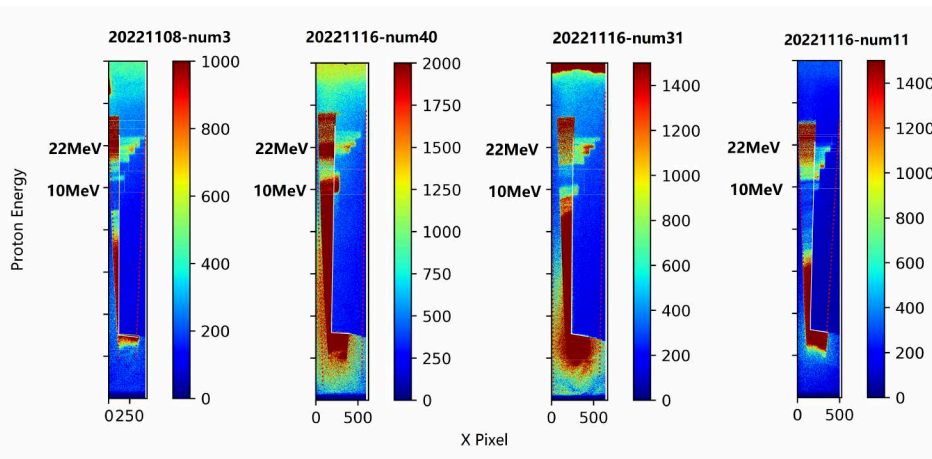
Fig. 2: The raw energy spectrum of circularly polarized light incident on the 40 nm target. The laser intensities are around num3: 2 \times 10^{21} \text{W/cm}^2 , num40: 1.7 \times 10^{21} \text{W/cm}^2 , num31: 1.4 \times 10^{21} \text{W/cm}^2 , and num11: 1.1 \times 10^{21} \text{W/cm}^2 , respectively.
