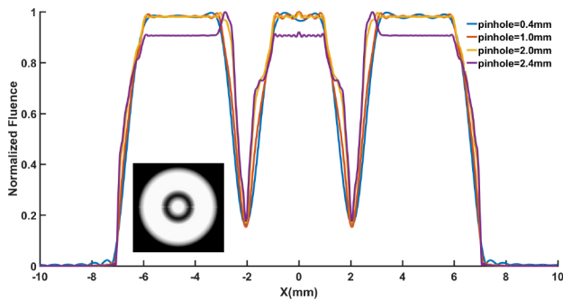
Fig. 3.14: Comparing different pinhole sizes for double-ring aperture. Due to the diffraction effect of light, the beam cannot be completely blocked. Inset for 2D light profile.
