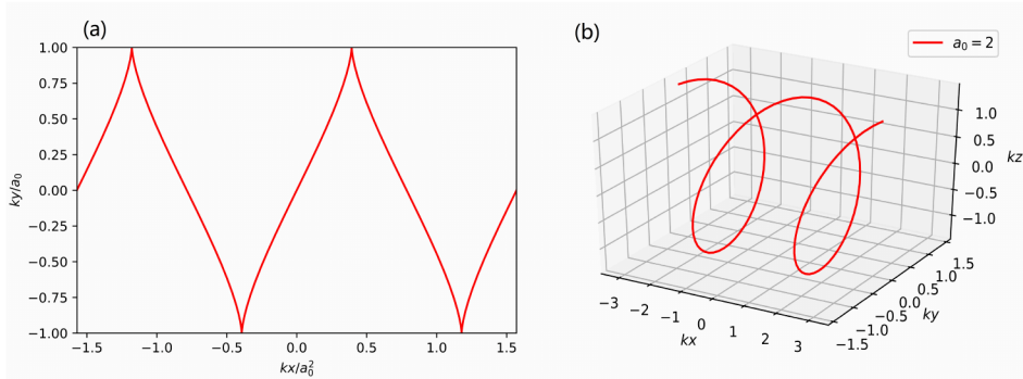
Fig. 2.3: (a) and (b) correspond to the trajectories of electrons in linearly and circularly polarized plane waves.
