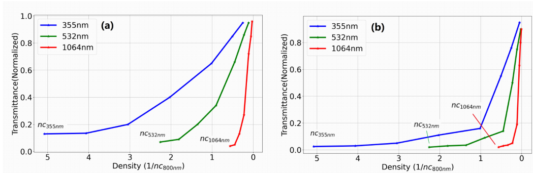
Fig. 6.4: Numerical calculation results of probe light transmittance as a function of peak plasma densities. The initial target is 30 nm. (a) The pre-pulse intensity is 5 \times 10^{13} \text{W/cm}^2 , and (b) The pre-pulse intensity is 3 \times 10^{15} \text{W/cm}^2 . The plasma density has been normalized by n_{C800nm} .
