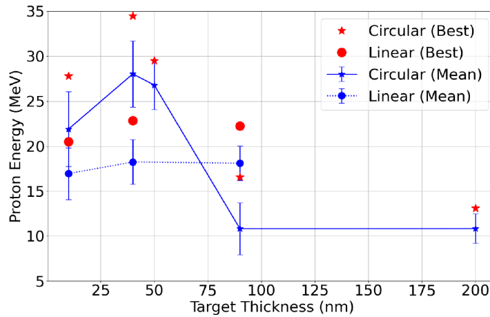
Fig. 5.2: The target thickness scan with circular and linear polarization laser. The mean value and the best data are shown for each thickness.
