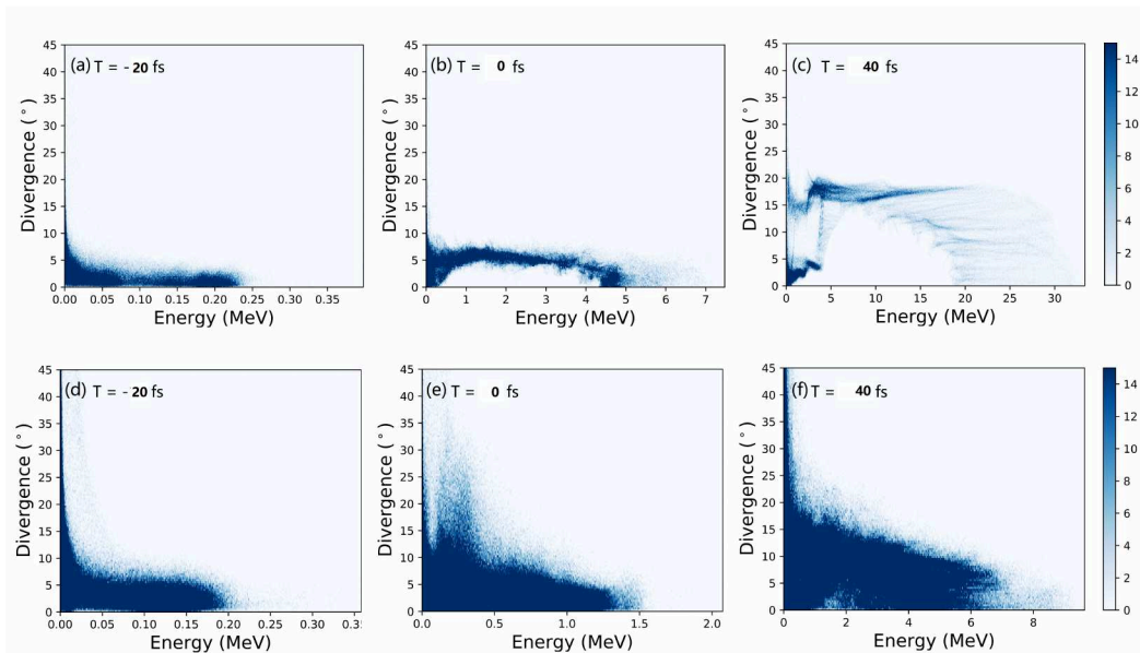
Fig. 5.10: The divergence angle distributions of the 40 nm and 90 nm target proton beams at different times are shown respectively. (a) - (c) and (d) - (f) correspond to the results for 40 nm and 90 nm targets, respectively.
