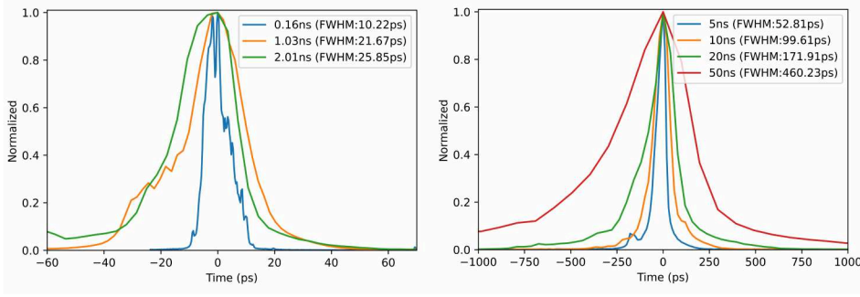
Fig. 3.7: The response curves of the streak camera to a 25 fs laser was measured at various sweeping times using a 40 \mu\text{m} slit. The sweeping time of the streak camera ranges from 0.16 ns to 50 ns, with the FWHM of the corresponding output image enclosed in brackets.
