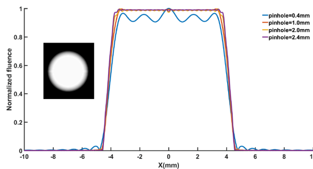
Fig. 3.12: Comparison of single ring aperture with different pinhole sizes. Inset for 2D light profile.
