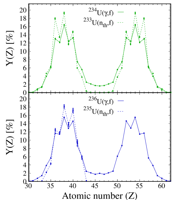
Figure 2. For the fissioning nuclei ^{234,236}\text{U} , results are also compared to thermal-neutron-induced fission of ^{233,235}\text{U} (dashed lines) from [7, 8], respectively.
