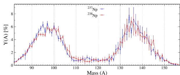
Figure 5. Experimental isobaric yields, with their uncertainties, measured for ^{237,238}\text{Np}(\gamma, f) with the R 3 B/SOFIA setup.
