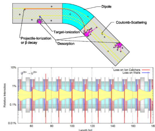
Figure 1: Top: Charge exchange processes at collisions with residual gas particles drive local pressure bumps. Bottom: The SIS100 charge separator lattice provides a peaked loss distribution for ionized projectiles with peaks in the middle of each doublet group (red lines). This loss distribution enables a control of the desorbed gases.
