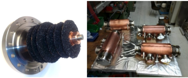
Figure 3: Left: Cryosorption pump using charcoal for H 2 and He-pumping. Right: Series cryogenic ion catchers with included low desorption beam absorbers.
