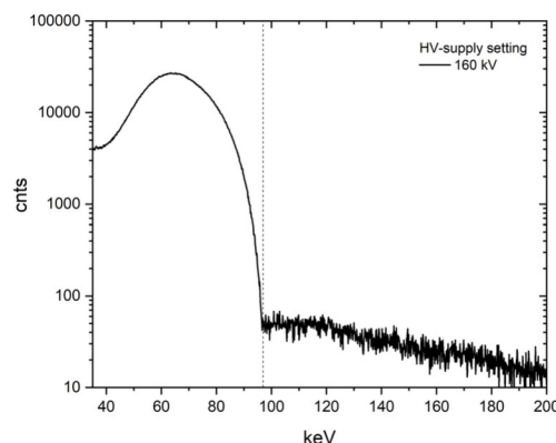
Figure 4: X-ray spectrum for the first measurement at the extraction septum. High-energy cut-off at about 98 keV.
