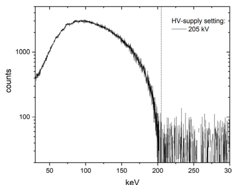
Figure 5: X-ray spectrum at the injection septum. The high-energy cut-off corresponds to the voltage setting.
