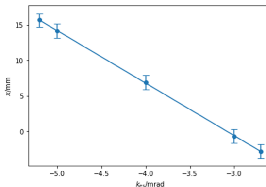
Figure 3: Deflection of beam by changing nominal extraction septum angle, as observed by beam position at a viewing screen after the magnetic extraction septum.
