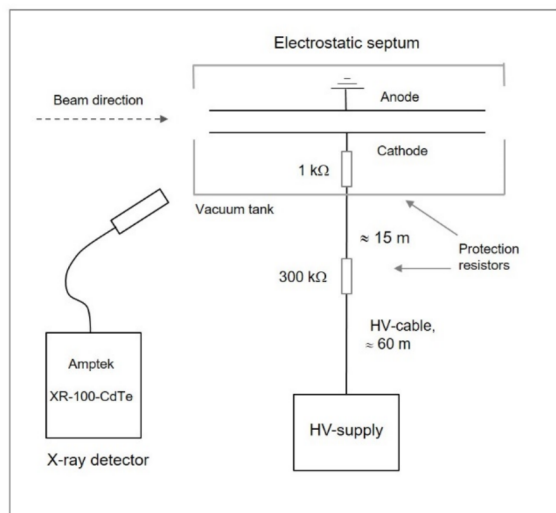
Figure 2: Schematic measurement set-up, with the X-ray detector at the upstream flange of the electrostatic septum.
