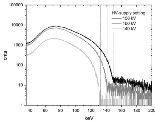
Figure 6: X-ray spectrum with new HV-supply, three different voltage settings.
