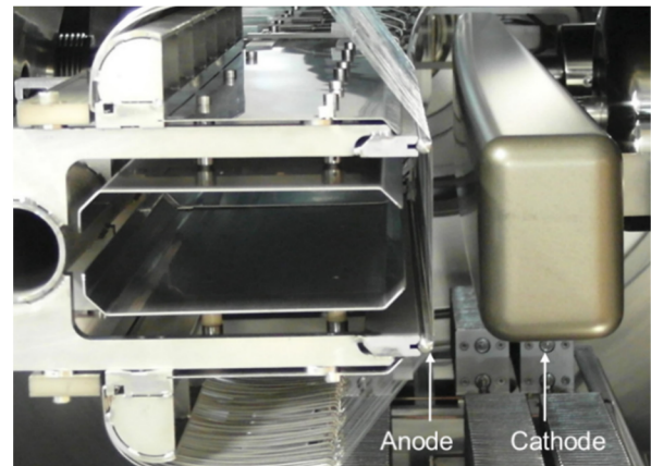
Figure 1: The electrostatic extraction septum in the beam direction with the anode wires and the cathode pointed out. The circulating beam area is to the left, and the extraction channel is to the right between the anode wires and the cathode.
