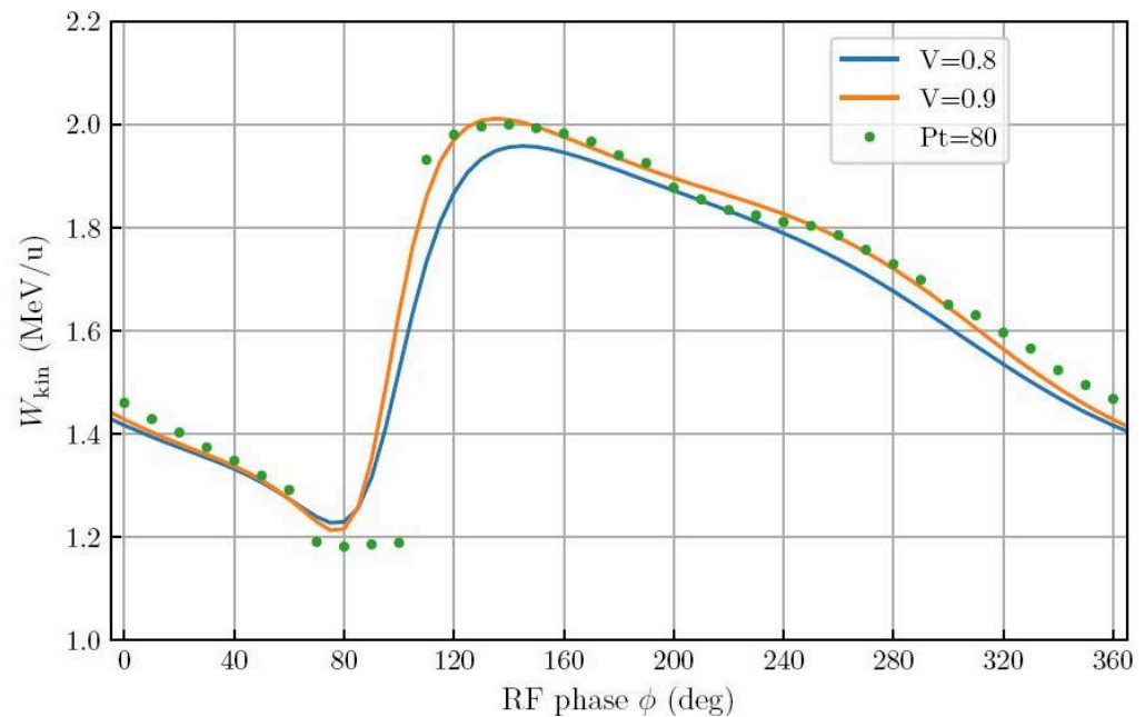
Figure 3. \text{Ar}^{9+} beam energy W_{kin} behind the first HELIAC cavity, powered at P_t = 80 mW, as a function of the rf-phase \Phi (dotted line). The corresponding simulation results are shown for 80% and 90% of the design voltage V (solid lines).
