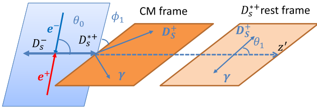
Fig. 2. Definition of the helicity frame for e^+e^- \rightarrow \gamma^* \rightarrow D_s^{*+}D_s^- , D_s^{*+} \rightarrow \gamma D_s^+ sequential decay.
