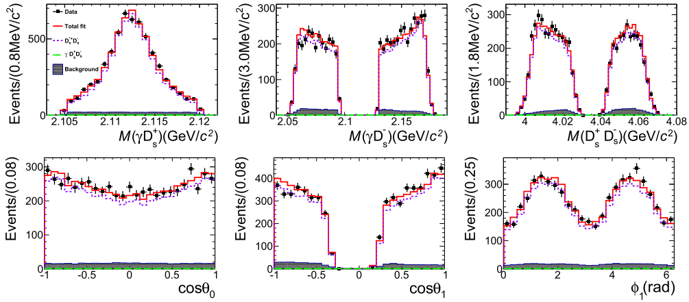
Fig. 3. Mass and angular distributions of D_s^{*+} tag sample for J^P = 1^- hypothesis. Points with error bars are data. The solid red line, dotted purple line, and long dashed green line are the total fit results, D_s^{*+} D_s^- , and \gamma D_s^{*+} D_s^- processes, respectively. The shaded black histograms indicate the scaled backgrounds derived from the inclusive MC samples.
