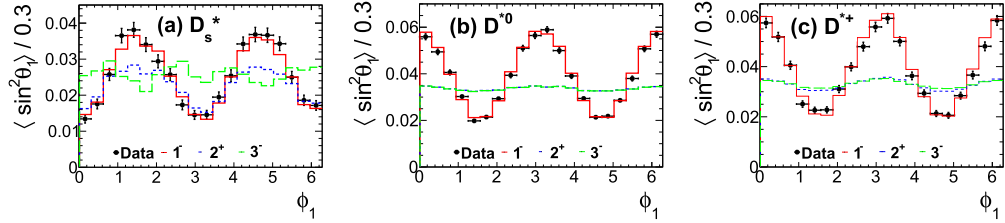
Fig. 4. Distributions of the normalized moment \langle \sin^2\theta_1 \rangle versus \phi_1 for the processes e^+e^- \rightarrow (a) D_s^{*+} D_s^- , (b) D^{*0} \bar{D}^0 and (c) D^{*+} D^- . Points with error bars are data summing over D^{*+} -tag sample and D -recoil sample with background events subtracted. The solid red line, dotted blue line, and the long-dashed green line are the fit results for the J^P = 1^- , 2^+ , and 3^- hypothesis, respectively. For the (b) and (c) processes, the blue line is hidden below green line.
