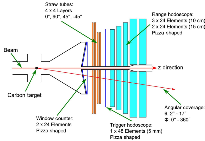
FIG. 1. Cross-sectional diagram showing the layout of the WASA forward detector, reprinted from Ref. [58]. The beam travels from left to right (horizontal red arrow), closely passing a 2-cm-thick carbon block target along the way. The beam is heated vertically to bring beam particles to the front face of the target. Scattered particles moving forward exit the vacuum through a stainless steel window at angles between 2^\circ and 17^\circ . They then pass through two plastic scintillator window counters cut into pie-shaped segments, an array of straw tubes for position and angle tracking, a segmented trigger hodoscope, and five layers (light blue) of plastic scintillator calorimeter detectors. The trigger counter and calorimeter detectors are also divided into pie-shaped segments. All the scintillator counters are read out using photo-multiplier tubes mounted at the outer edge of each pie segment.
