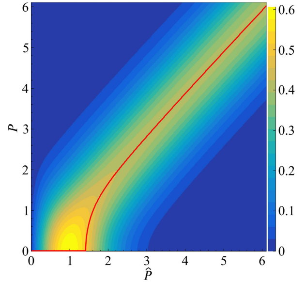
FIG. 11. A two-dimensional Rice plot for one cycle. The red line represents the value of P for which Eq. (30) is maximum for a given value of \hat{P} .
