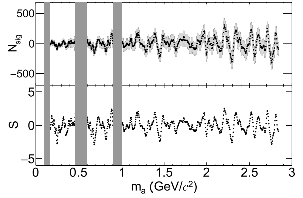
Fig. 4. The distribution of the signal yields N_{\text{sig}} (upper plot) and the local significance S (lower plot) obtained from the maximum-likelihood fits as a function of m_a . The vertical gray bands indicate the excluded regions close to the \pi^0 , \eta , and \eta' masses.
