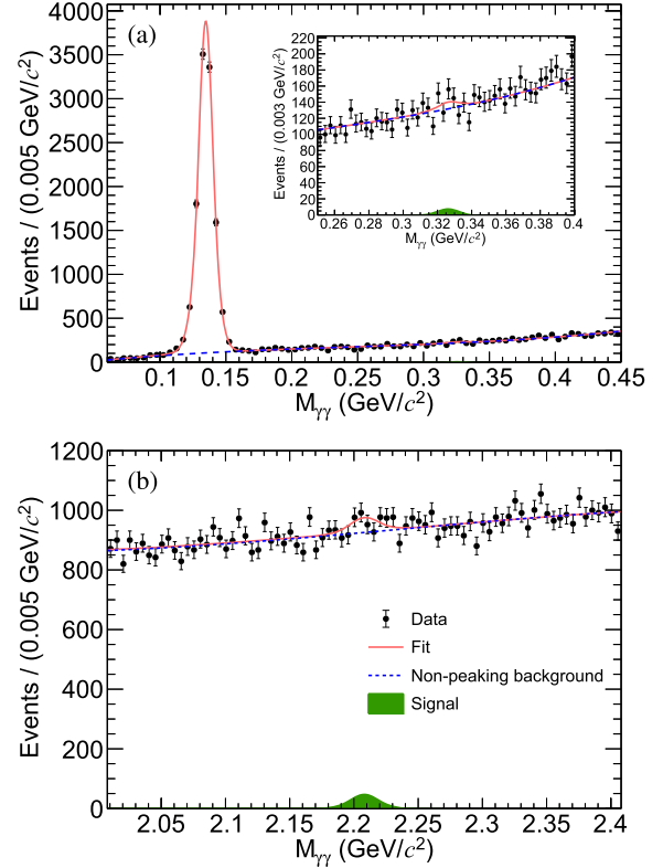
Fig. 3. The M_{\gamma\gamma} distribution for (a) m_a = 0.327 GeV/c 2 and (b) m_a = 2.208 GeV/c 2 with the fit results overlaid. The black dots with error bars are data, and the contribution of the non-peaking background is represented by a blue dashed curve. The green shaded region and the red solid curve represent the signal PDF and the total PDF, respectively. The inset of the figure (a) displays an enlargement of the M_{\gamma\gamma} region between 0.25 and 0.4 GeV/c 2 . The largest local significance is 2.6 \sigma at the m_a = 2.208 GeV/c 2 hypothesis.
