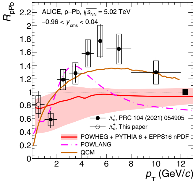
FIG. 4. Nuclear modification factor R_{pPb} of prompt \Lambda_c^+ baryons in p -Pb collisions at \sqrt{s_{NN}} = 5.02 TeV as a function of p_T , compared with model calculations [59,60,63,64].
