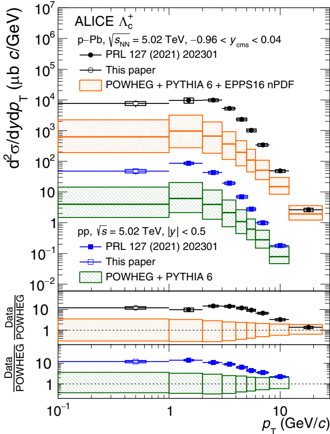
FIG. 3. The p_T -differential \Lambda_c^+ production cross sections in pp and p -Pb collisions at \sqrt{s_{NN}} = 5.02 TeV [12], including the new measurements in 0 < p_T < 1 GeV/c as open markers. The lower panels show the ratios of the measurements to POWHEG+PYTHIA6, with EPPS16 nPDF calculations included for p -Pb collisions [9,59,60].
