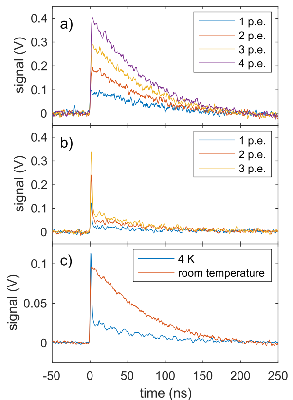
FIG. 4. (a) Oscilloscope traces of SiPM pulses at room temperature and a bias voltage of 26.5 V. (b) Oscilloscope traces at 4 K and a bias voltage of 24.0 V. In (a) and (b), one graph for each n -photoelectron pulse is shown. (c) Direct comparison of the SiPM pulse shape at 4 K and room temperature. The average of 27 one-photoelectron pulses is plotted for both temperatures. p.e.: photoelectron.
