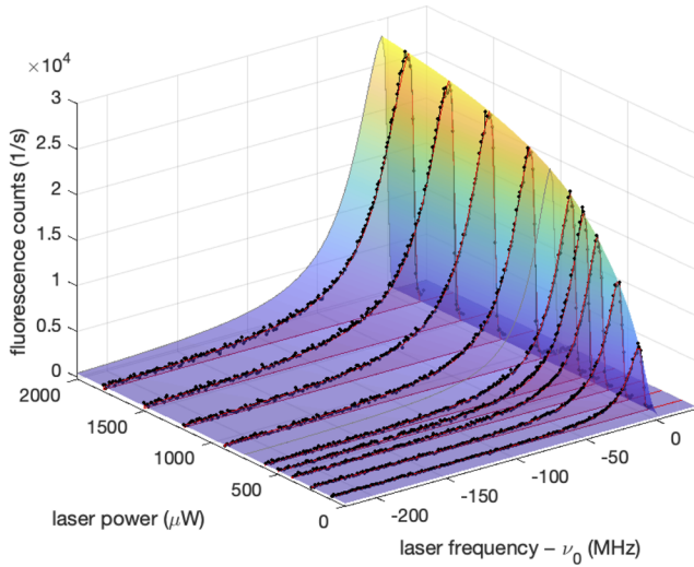
FIG. 11. Fluorescence spectra of run 2 with 5100(200) ions. Description as in Fig. 10. In run 2, we observe a reduced background count rate of 6–7 s −1 per μW, compared to 250–1300 s −1 per μW in run 1, due to stray light suppression. In addition, stabilization of the laser power in run 2 leads to a background count rate, which is independent of the laser frequency. Furthermore, the laser frequency is stabilized to 2 MHz peak-to-peak fluctuation, compared to ≈20 MHz in run 1. Finally, in run 2, no RF drive is applied, which eliminates line-broadening effects and allows for a better temperature estimate.
