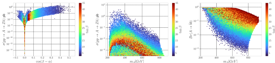
Figure 1. The scan output points that satisfy all constrains. (Left) Total cross section of the process pp \rightarrow A \rightarrow Zh at \sqrt{s} = 14 GeV versus \cos(\beta - \alpha) . (Middle) The same versus m_A . (Right) The decay rate Br(A \rightarrow b\bar{b}) versus m_A . The color bar represents the corresponding \tan\beta value in all plots.
