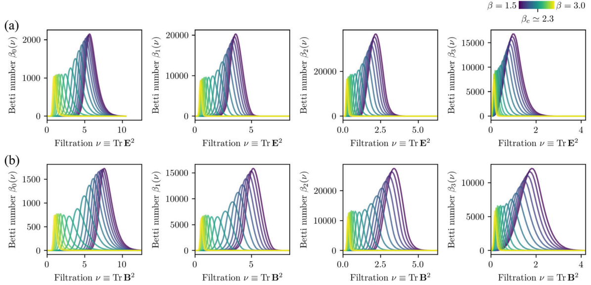
FIG. 15. Betti number distributions in dimensions zero to three of (a) \text{TrE}^2 and (b) \text{TrB}^2 superlevel set filtrations for cooled configurations. Data is given in lattice units.
