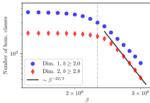
FIG. 6. Number of homology classes in the angle difference filtration constructed from \phi(\mathbf{x}) = \arg(\text{Tr}\mathcal{P}(\mathbf{x})/2) with birth b \geq 2.0 for dimension one and b \geq 2.8 for dimension two, compared to the semiclassical one-loop instanton appearance probability scaling behavior \sim \beta^{-22/3} .
