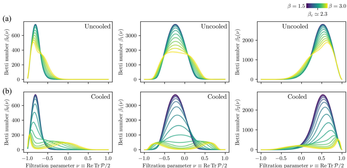
FIG. 3. Betti number distributions of dimensions zero to two for the sublevel set filtration of P(\mathbf{x}) = \text{Tr}\mathcal{P}(\mathbf{x})/2 for (a) uncooled and (b) cooled configurations.
