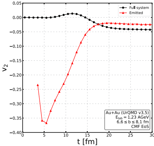
Fig. 2. The elliptic flow coefficient v_2 calculated from all baryons (black circles) which are present in the whole phase space at time t and of the nucleons emitted at time t + \Delta t (red triangles) from 20–30% peripheral Au+Au collisions at a kinetic beam energy of 1.23A GeV from UrQMD.
