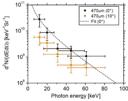
FIG. 13. Spectrum of betatron radiation in the directions of 0^\circ and 10^\circ evaluated with a help of thick filters.
