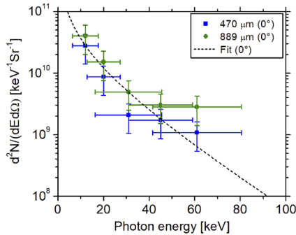
FIG. 15. X-ray spectra from shots evaluated with the help of the thick filters placed at 0° to the laser axis.
