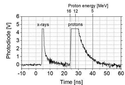
(a) without proton/ion shielding
