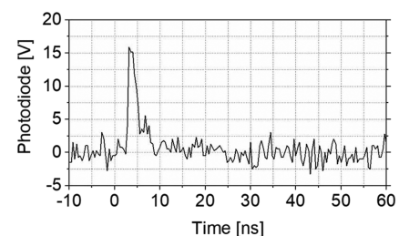
(b) proton/ion shielding: 560 \mu\text{m} thick Mylar foil
