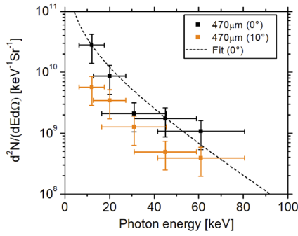
FIG. 13. Spectrum of betatron radiation in the directions of 0° and 10° evaluated with a help of thick filters.
