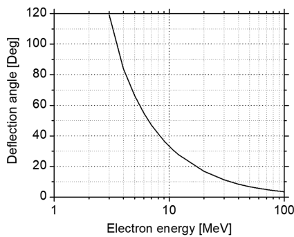
FIG. 10. Deflection of electrons by the magnetic yoke as a function of electron energy.
