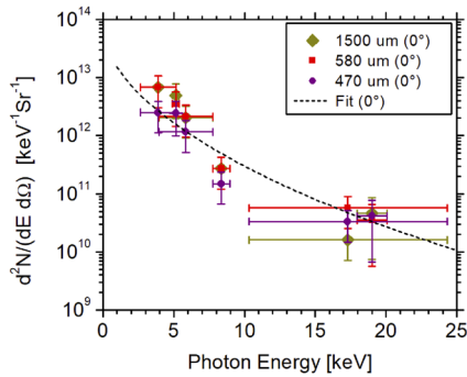
FIG. 14. X-ray spectra for different 2 mg/cm 3 foam thicknesses evaluated with the help of the thin filters set placed at 0° to the laser axis.
