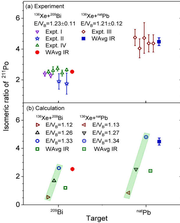
Fig. 4. (a) IRs of ^{211}\text{Po} produced in ^{136}\text{Xe}+^{209}\text{Bi} at E/V_B=1.23\pm0.11 and ^{136}\text{Xe}+^{\text{nat}}\text{Pb} at E/V_B=1.21\pm0.12 corresponding to 945 MeV beam energy in different experiments. Details of the experimental parameters are described in Table 1. (b) Estimation of IRs of ^{211}\text{Po} at three projectile energies and comparison of WAvG of IRs with measured results for ^{136}\text{Xe}+^{209}\text{Bi} and ^{136}\text{Xe}+^{\text{nat}}\text{Pb} . WAvG refers to the Weighted Average. Strip lines are shown as a guide to the eye for increasing IRs with projectile energy.
