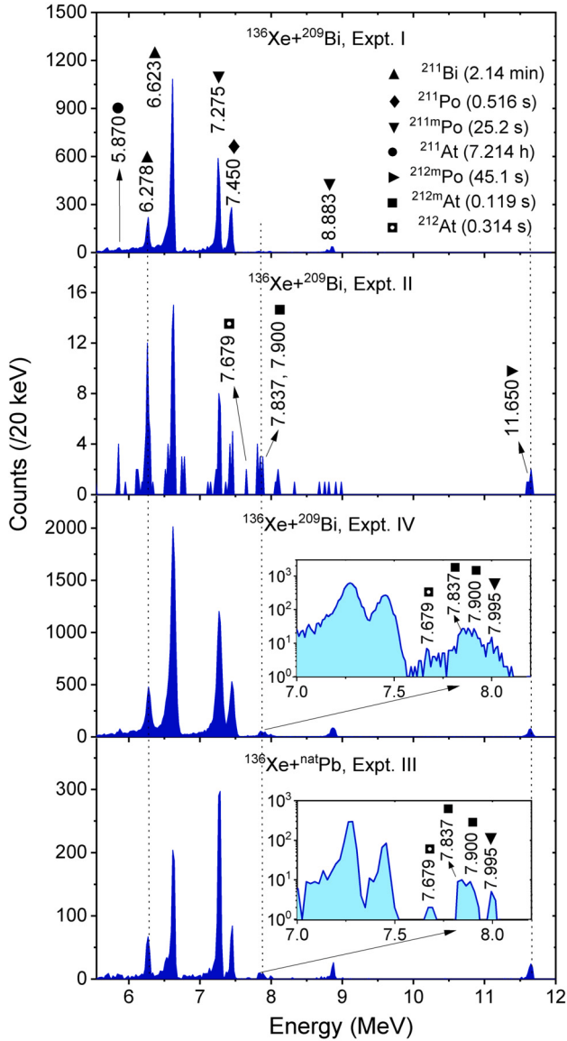
Fig. 2. Characteristics \alpha -decay spectra of TLFs measured in three independent experiments using ^{136}\text{Xe} + ^{209}\text{Bi} at E/V_B = 1.23 \pm 0.11 and one with ^{136}\text{Xe} + \text{natPb} at E/V_B = 1.21 \pm 0.12 for different gas cell configurations.
