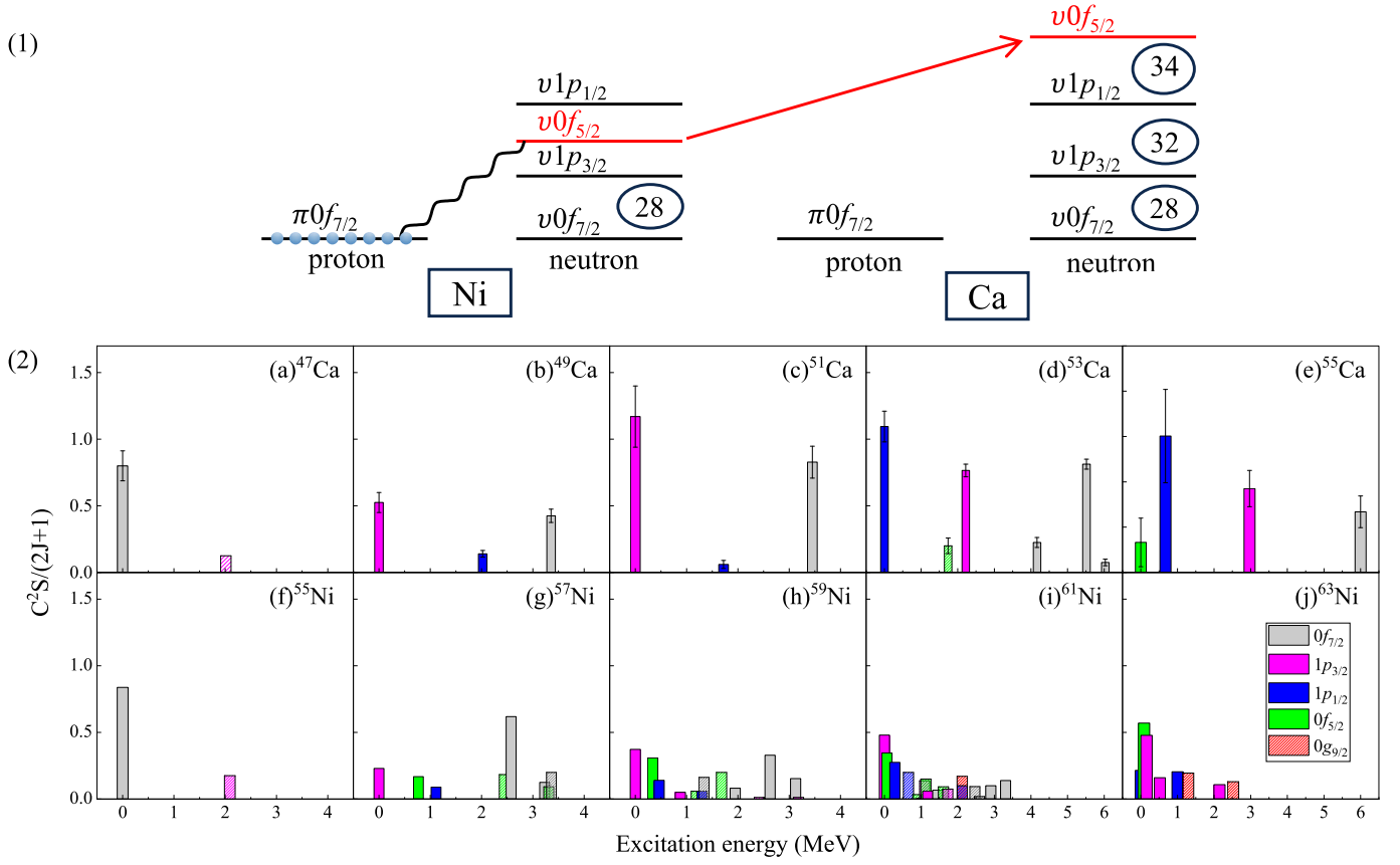
Fig. 7. (1) Schematic illustration of shell evolution from Ni to Ca for neutron pf orbitals. The wavy line implies the attractive interaction between the proton 0f_{7/2} and the neutron 0f_{5/2} orbits. Adopted from Ref. [61]. (2) Normalized spectroscopic factors of neutron-hole states as a function of excitation energy in the Ca ( Z = 20 ) and Ni ( Z = 28 ) isotopes, populated from neutron removal reaction. Data of Ca isotopes are taken from neutron knockout reactions [6,2,5,17] and the present work (unbound states); Data of Ni isotopes are taken from ( p , d ) or ( ^3\text{He} , \alpha ) transfer reactions [62,63]. Values where C^2S/(2J+1) < 0.05 have been multiplied by a factor of 5 and are displayed with hatching in the color corresponding to the respective orbital.
