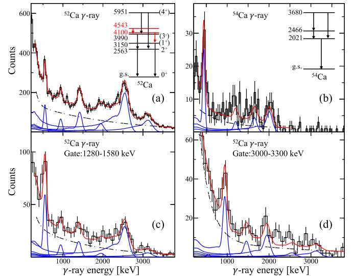
Fig. 1. Doppler-corrected de-excitation \gamma -ray spectra of ^{52,54}\text{Ca} fragments following neutron decays. (a) and (b) show the total spectra for ^{52}\text{Ca} and ^{54}\text{Ca} , respectively. The fit function (red line) comprises a double-exponential background and 14.0(20) %, respectively. (c) and (d) show the two new \gamma -ray transitions in the ^{52}\text{Ca} spectra obtained in coincidence with the closest 1427-keV transition and 3150-keV transition, respectively.
