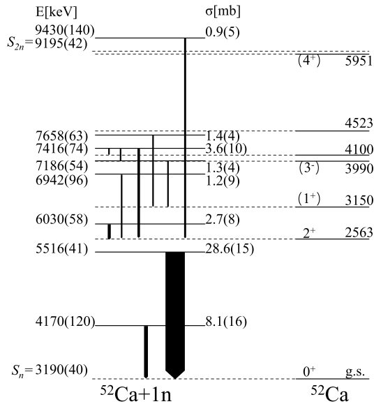
Fig. 3. Partial level scheme of unbound states in ^{53}\text{Ca} following the ^{54}\text{Ca}(p, pn) reaction. The position and width of the unbound states were reconstructed from a detailed analysis of decay neutrons in coincidence with \gamma rays. Arrow widths represent the relative intensity. Bound states of ^{53}\text{Ca} were omitted.
