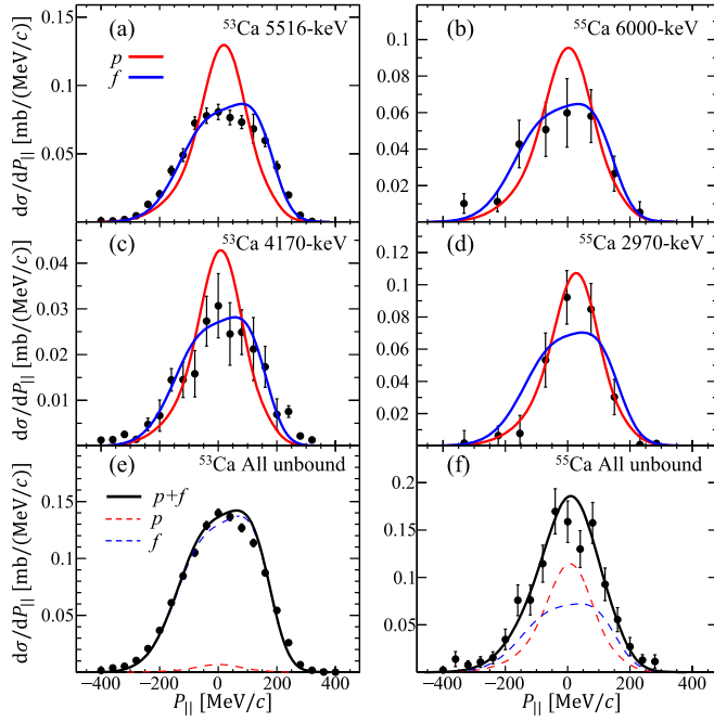
Fig. 5. Exclusive parallel momentum distributions for (a) 5516-keV and (c) 4170-keV states of ^{53}\text{Ca} , (b) 6000-keV and (d) 2970-keV states of ^{55}\text{Ca} . Solid curves are the calculated DWIA predictions assuming an 1n knockout from p and f orbitals and have been normalized to experimental cross-sections. Panel (e) and (f) display PMDs for all the unbound states of ^{53}\text{Ca} and ^{55}\text{Ca} , respectively, compared with a linear fit (black, solid lines) between p -curve (red, dashed) and f -curve (blue, dashed). Error bars represent statistical errors.
