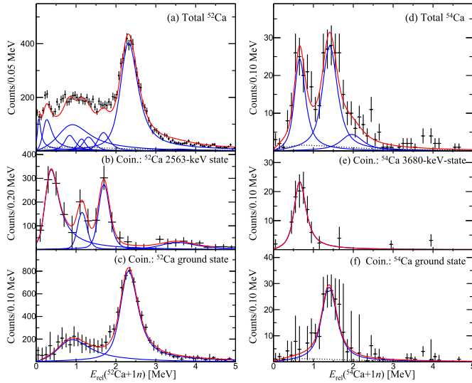
Fig. 2. (a) Relative energy spectrum of ^{54}\text{Ca}(p, pn)^{53}\text{Ca} \rightarrow ^{52}\text{Ca} + 1n ; Exclusive relative energy spectra in coincidence with the 2563-keV state (b) and the ground state (c) in ^{52}\text{Ca} . (d) Relative energy spectrum of ^{56}\text{Ca}(p, pn)^{55}\text{Ca} \rightarrow ^{54}\text{Ca} + 1n ; Exclusive relative energy spectra in coincidence with the 3680-keV state in ^{54}\text{Ca} (e), and ground state (f). The overall fit function (red line) comprises the sum of the simulated responses of NeuLAND + NEBULA and beamline detectors (blue lines), and a non-resonant background (black long-dashed line).
