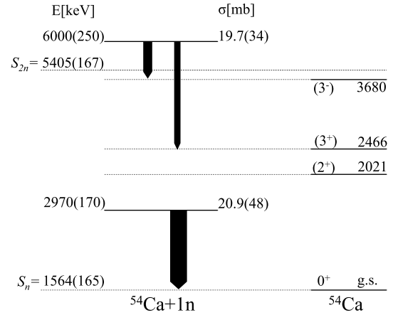
Fig. 4. Same as Fig. 3, but for unbound states in ^{55}\text{Ca} following the ^{56}\text{Ca}(p, pn) reaction.
