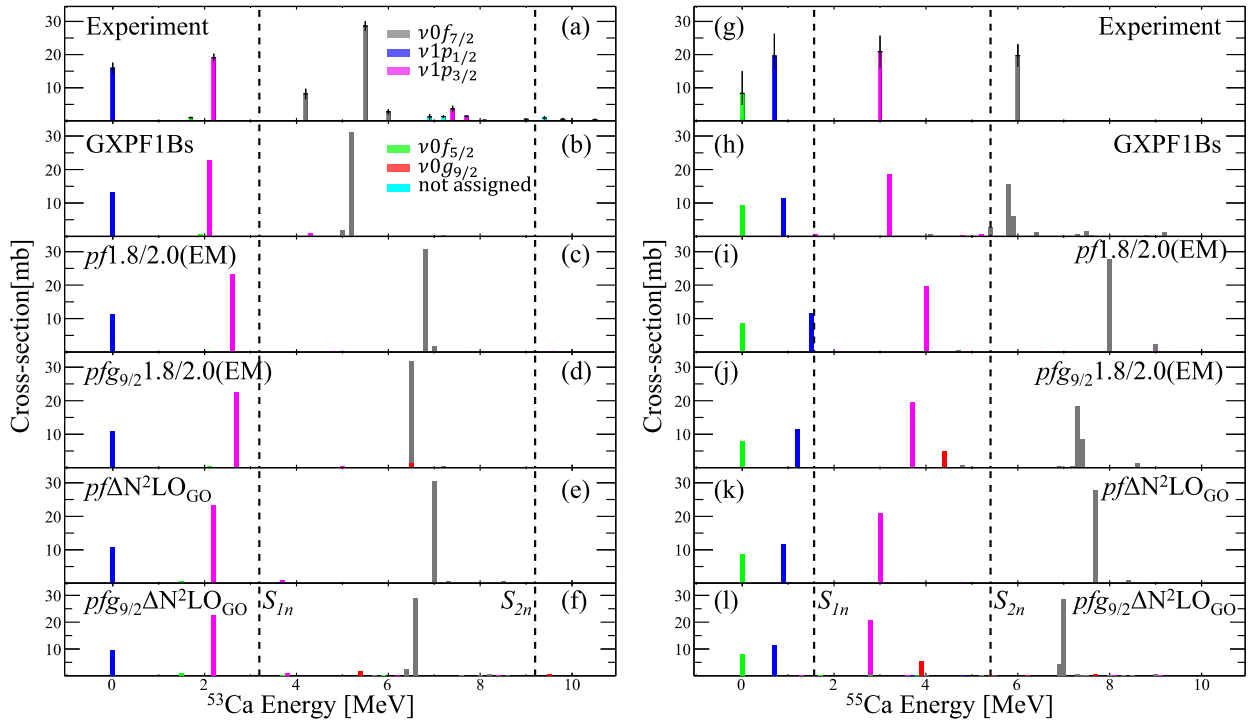
Fig. 6. Panels (a) and (g) depict the measured cross-sections for ^{53}\text{Ca} and ^{55}\text{Ca} as a function of excitation energy. The cross-sections to bound states below S_{1n} were deduced from \gamma -ray spectroscopy measurements [5,17]. The cross-sections to the unbound states (this work) were obtained from invariant mass spectroscopy. Identified neutron-hole states are colored accordingly to the orbital of the removed neutron. The other states with no conclusive PMDs are labeled “not assigned”. Panels (b-f) are the theoretical predictions of energies and cross-sections. Predictions associated with the v0g_{9/2} orbital are scaled by a factor of 5.
