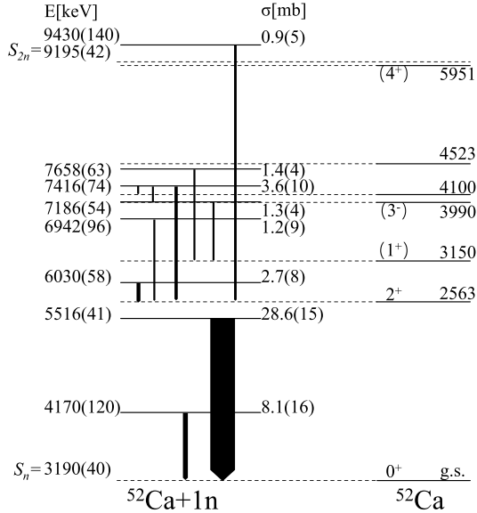
Fig. 3. Partial level scheme of unbound states in ^{53}\text{Ca} following the ^{54}\text{Ca}(p, pn) reaction. The position and width of the unbound states were reconstructed from a detailed analysis of decay neutrons in coincidence with \gamma rays. Arrow widths represent the relative intensity. Bound states of ^{53}\text{Ca} were omitted.
