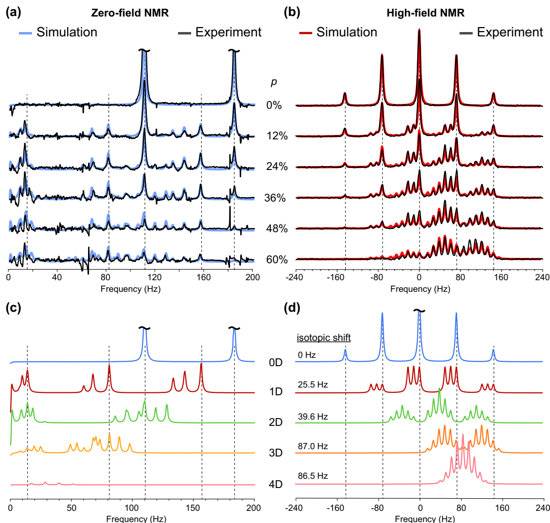
Fig. 4 | Zero- and high-field spectra of ammonium isotopologues with varying deuterium concentration. Experimentally measured (a) zero-field NMR spectra and (b) high-field (18.8 T) ^{15}\text{N} NMR spectra of \text{H}_2\text{O}/\text{D}_2\text{O} solutions containing a mixture of isotopologues of ammonium, ^{15}\text{ND}_x\text{H}_{4-x}^+ , prepared by varying the molar
