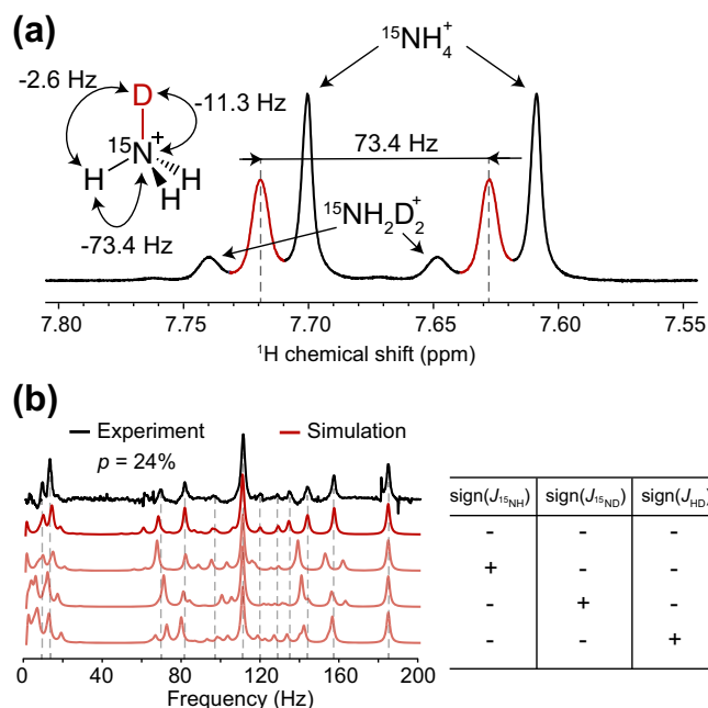
Fig. 5 | Zero-field NMR spectroscopy allows the direct extraction of the sign of J -couplings. a ^1\text{H} NMR spectrum (800 MHz) and (b) ZULF NMR spectrum (black) of ^{15}\text{ND}_x\text{H}_{4-x}^+ solution with deuterium fraction p = 24\% . In (b) , calculated zero-field J -spectra of a mixture of isotopologues is shown in red, corresponding signs of J -couplings are presented on the right. Given insensitivity to global sign changes, only the four non-redundant permutations from the total eight possible combinations of J -coupling signs are shown.
