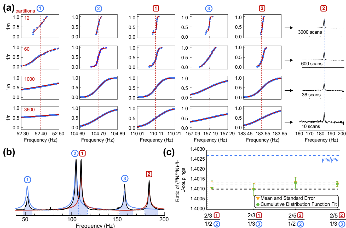
Fig. 2 | Statistical analysis of the J -coupling ratio of the ammonium isotopologues. a Positions of the maxima extracted from peaks corresponding to isotopologues of ammonium organized in the ascending order ( 1/n where n is a partition number) generate cumulative distribution functions (CDFs); the averaged spectra with 3000, 600, 36, and 10 scans correspond to 12, 60, 1000, and 3600 partitions, respectively. b Zero-field NMR spectrum of [^{14}\text{N}] - and [^{15}\text{N}] -ammonium
