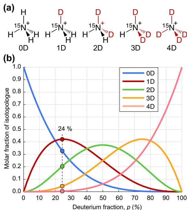
Fig. 3 | The deuterium concentration in the samples studied in this work follows a binomial distribution. a Isotopologues of the ammonium cation ( ^{15}\text{ND}_x\text{H}_{4-x}^+ ) are present in the aqueous solution. The fraction of deuterium was varied by changing the amount of \text{H}_2\text{O} vs. \text{D}_2\text{O} . Isotopologues are labeled x\text{D} where x represents a number of deuterium atoms in the molecule. b Equilibrium molar fractions of the isotopologues as a function of deuterium fraction in solution as determined by Eq. (1).
