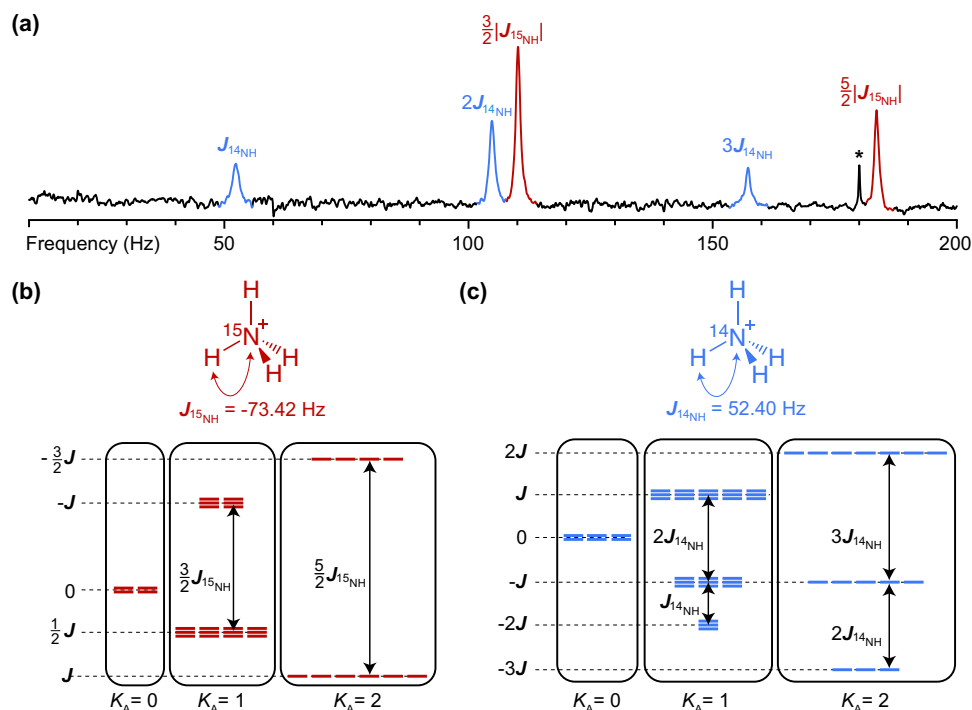
Fig. 1 J -spectra and energy levels of the ammonium isotopologues studied in this work. a Zero-field NMR J -spectra of the mixture of [ 15 N]- and [ 14 N]-ammonium cations ( 15 NH 4 + and 14 NH 4 + ) in aqueous solution of H 2 SO 4 (2 M). The asterisk depicts the third harmonic of the 60 Hz power-line frequency. b, c Molecular diagram and nuclear spin energy-level structure of the [ 15 N]-ammonium and [ 14 N]-ammonium
