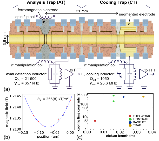
FIG. 1. (a) Double trap system, consisting of a cooling trap (CT) and an analysis trap (AT), with a superimposed magnetic bottle with a strength of B_{2,AT} = 266(8) kT/m 2 . The CT is equipped with a resonant cooling resistor to thermalize the modified cyclotron mode. To the end-cap electrode of the AT an Q \approx 21\,500 superconducting detection system at 657 kHz is connected, providing optimum frequency measurement performance at the given trap and detector geometry. (b) Magnetic field in the center of the AT. (c) Comparison of cooling time constants for different trap experiments. Our experiment is operated at \tau_{+,CT} \approx 4.5 s, more than 10 \times faster than other state-of-the-art trap experiments.
