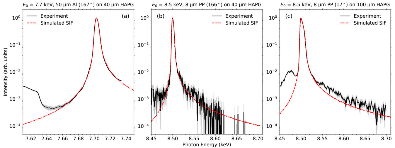
FIG. 7. A comparison of the crystal IF model (red dashed) fitted to experimental measurements (black) of the quasi-elastic signal of a monochromated beam with (a) E_0 = 7.7 keV on 50\text{ }\mu\text{m} thick Al with 40\text{ }\mu\text{m} HAPG, (b) E_0 = 8.5 keV on 8\text{ }\mu\text{m} thick polypropylene (PP) with 40\text{ }\mu\text{m} HAPG, and (c) E_0 = 8.5 keV on 8\text{ }\mu\text{m} thick PP with 100\text{ }\mu\text{m} HAPG. The angles in the brackets are the scattering angles at which the spectra were taken. The gray shaded regions indicate the uncertainty in the experimental spectra. The theoretical SIFs are plotted on energy axes that extend beyond the experimental spectral range of the detector.
