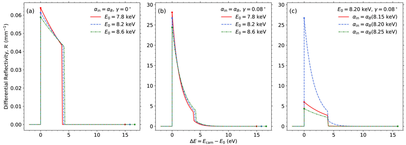
FIG. 2. The differential reflectivity from depth broadening in three scenarios involving a 40 \mu\text{m} thick graphite crystal, considering up to p = 4 reflections. Note the marked increase in reflectivity when mosaicity is taken into account. In all cases, the circular markers indicate the energy difference on detector that a photon can be reflected to. (a) Depth broadening for a photon with different energies incident at its Bragg angle on a crystal without mosaicity. Note that the shift on the detector is only for \Delta E > 0 and that the maximum \Delta E is different for each photon energy. (b) The same as (a), but now the crystal has a mosaicity \gamma = 0.08^\circ . (c) Depth broadening for a fixed photon energy on a mosaic crystal at different angles of incidence.
