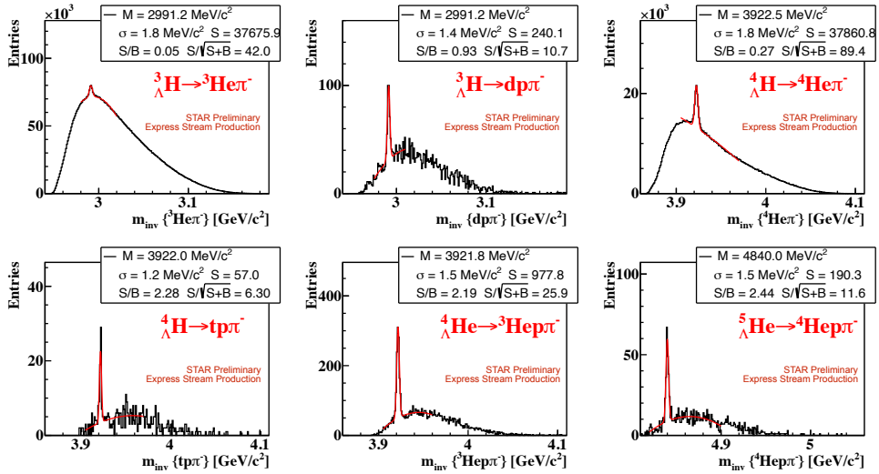
Figure 3. Standard and express reconstruction of hypernuclei using 2018, 2019, 2020, and 2021 data collected at different energies in the collider and fixed-target modes. The signal of {}^5_{\Lambda}\text{He} is visible with a significance of 11.6\sigma .
