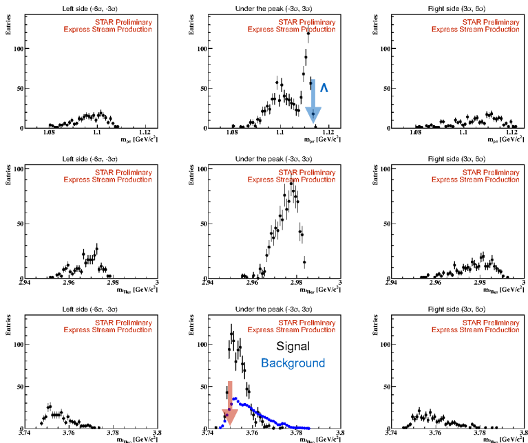
Figure 5. Projections of the Dalitz plots for the decay {}^4_{\Lambda}\text{He} \rightarrow {}^3\text{He} + p + \pi^- . The complex structure in the p\pi^- projection can be explained as a possible spin effect. In the nucleus- p combination, the signal and the background show different behavior. There can be seen a hint of two-body {}^4\text{Li} \pi^- decay ( {}^4\text{Li} (J^P = 2^-) : M = 3.75 \text{ GeV}/c^2 , \sigma = 8.7 \text{ MeV}/c^2 ).
