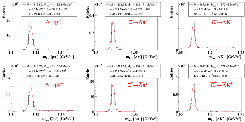
Figure 2. With express calibration and production we observe in real time all hyperons with high significance and S/B ratio (140M AuAu events at 7.7 GeV, 2021).
