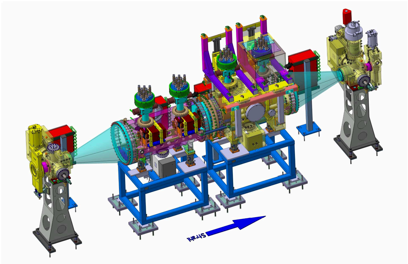
Figure 2: Design of the HESR injection kicker system. The system consist of four magnets inside of two vacuum tanks. The tanks are delivered separately and connected together at place using special bellow. Each magnet is connected to semiconductor based pulser using six coaxial cables which are joint together in one HV feed-trough at the top of the vacuum tank. A lifting system is designed to prevent damages of the ceramic feed-trough due to the external forces at the cable and disconnect the systems from the pulsers for the time of the bake-out process. Special conical tubes are designed to smoothen injection section impedance for the particle beam. In addition to the turbo and ion pumps at each vacuum tank, there are also standard HESR pump systems installed at both sides of the kicker section.
