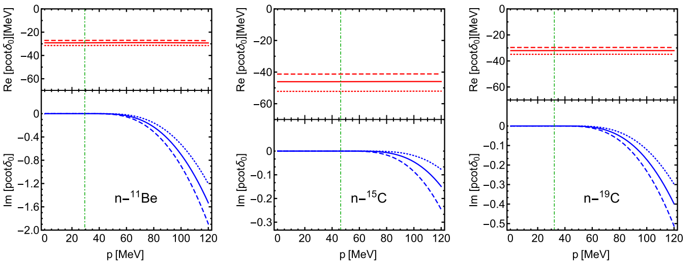
FIG. 6. Real and imaginary parts of p \cot \delta_0(p) for the s -wave scattering of neutron and one-neutron halo nuclei in the J = 1 channel. The left, middle, and right panels correspond to the n-^{11}\text{Be} , n-^{15}\text{C} , and n-^{19}\text{C} scattering processes, respectively. The solid lines represent the results using the scattering lengths a_\sigma in Table II as inputs, while the dashed/dotted curves correspond to a_\sigma \pm 0.5 fm, respectively. The vertical dot-dashed lines in the plots indicate the threshold for breakup into the neutron core continuum.
