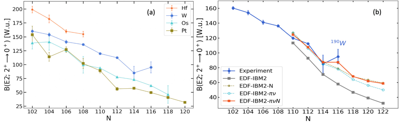
Fig. 7. (a) Experimental B(E2; 2^+ \rightarrow 0^+) values in even-even Hf, W, Os, Pt isotopes. The literature data was taken from Refs. [8–22]. (b) Comparison of experimental and theory B(E2; 2^+ \rightarrow 0^+) values for even-even tungsten isotopes.
