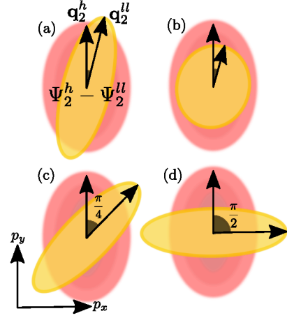
Figure 1: Sketch of the scalar product method 2, with the dilepton (hadron) event vector in yellow (red). See text for interpretation.
