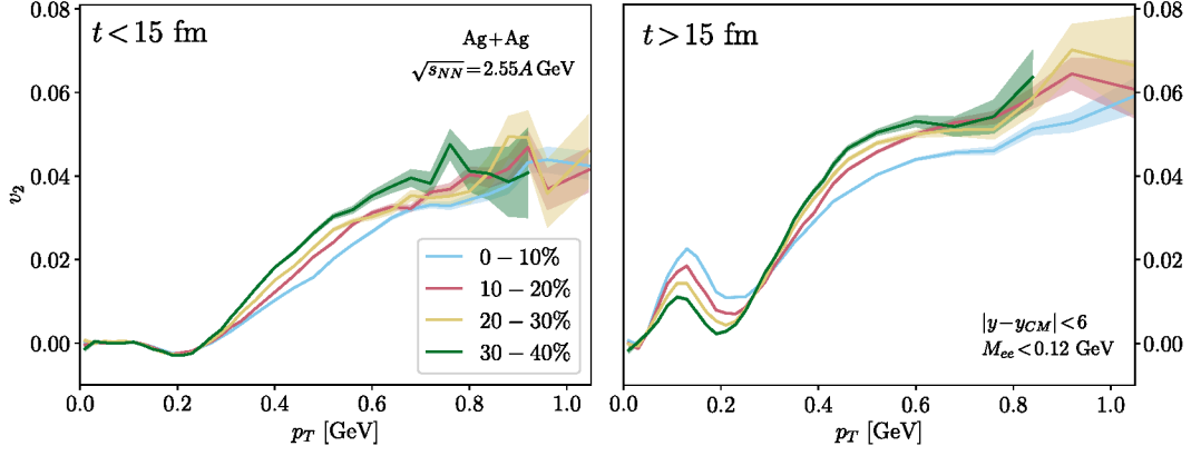
Figure 4: Dielectron v_2 as a function of p_T , for dileptons emitted (left) before and (right) after t = 15 fm.
