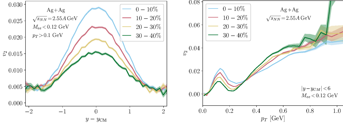
Figure 3: Same as Fig. 2, as a function of (left) rapidity y - y_{CM} and (right) transverse momentum p_T .
