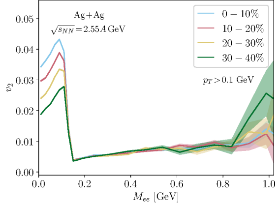
Figure 2: Dielectron v_2 as a function of invariant mass M_{ee} for Ag+Ag collisions at \sqrt{s_{NN}} = 2.55 in different centrality classes.
