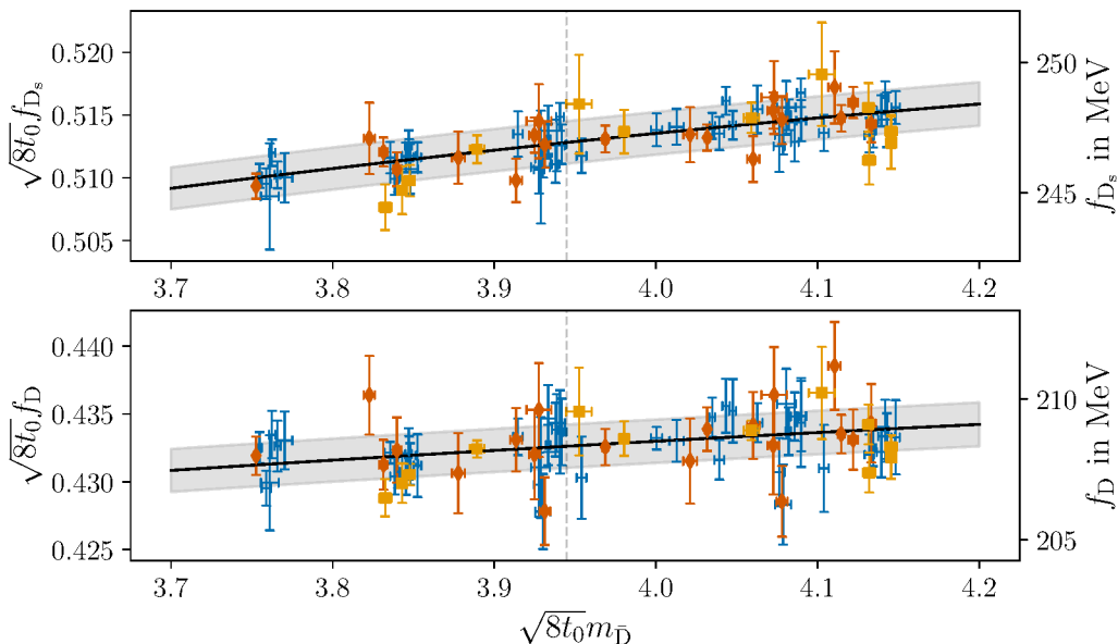
Figure 6. Dependence of f_{\text{D}} and f_{\text{D}_s} on the flavour average D meson mass for the fit with the largest AIC weight, as shown in figure 5. The dashed line indicates the physical value of \sqrt{8t_0}m_{\text{D}} . The data points are shifted using the fit to the physical pion and kaon masses and lattice spacing effects are removed. The central value and error for the corresponding m_{\text{D}} dependence of the fit are shown as the black line and grey band, respectively.
