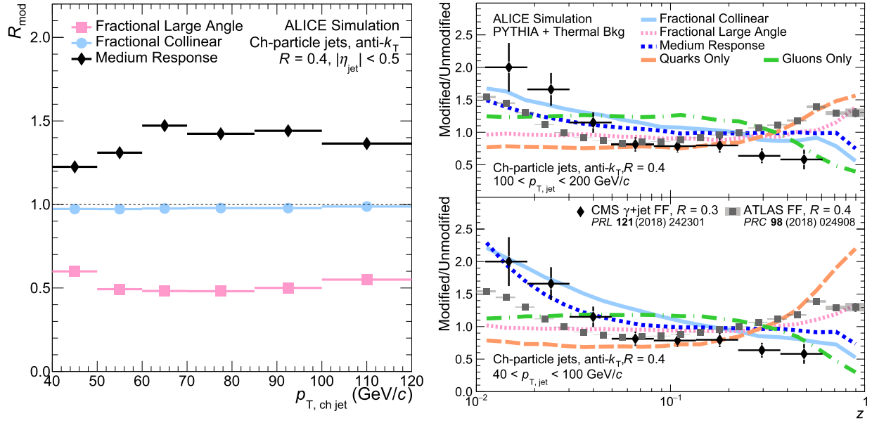
Fig. 2. Left: Comparison of toy model modifications for R = 0.4 jets using the R_{\text{mod}} as defined in Eq. (3) Right: The ratio of the modified to unmodified fragmentation functions at low jet p_T ( 40 < p_{T, \text{true}} < 100 GeV/c, lower right panel) and high jet p_T ( 100 < p_{T, \text{true}} < 200 GeV/c, upper right panel) for 0–10% central Pb–Pb collisions. In the fractional collinear and fractional large angle case, f_{\text{loss}} = 25\% and p_{\text{loss}} = 100\% . In the medium response case, f_{\text{loss}} = 10\% and p_{\text{loss}} = 50\% . The ratio of the fragmentation functions measured in Pb–Pb and pp collisions are shown for jets with R = 0.4 and p_T > 100 GeV/c [53] (ATLAS), and for jets with R = 0.3 and p_T > 30 GeV/c recoiling from a photon with E_T > 60 GeV/c [94] (CMS).
