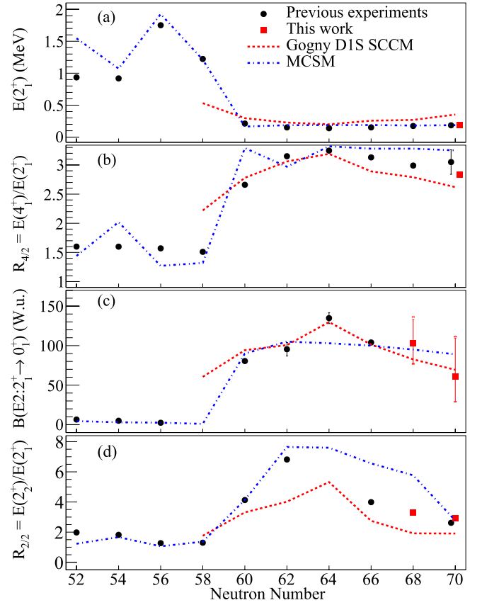
Fig. 4. Systematic plots of (a) E(2_1^+) , (b) R_{4/2} = E(4_1^+)/E(2_1^+) , (c) B(E2; 2_1^+ \rightarrow 0_1^+) , and (d) R_{2/2} = E(2_2^+)/E(2_1^+) values in Zr isotopes as a function of neutron number. Theoretical results from the SCCM [30] with the Gogny D1S interaction [37,38] and MCSM [16] calculations are shown to compare with the experimental data [11,5,39]. The error bars show the statistical uncertainties, while the caps represent the total errors including the systematic uncertainties, dominated by the atomic background subtraction.
