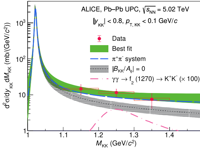
FIG. 2. Differential cross section of coherent K^+K^- photo-production as a function M_{KK} in Pb-Pb UPCs at \sqrt{s_{NN}} = 5.02 TeV in |y_{KK}| < 0.8 . The vertical lines and boxes along the data points represent statistical and systematic uncertainties, respectively. The green solid line presents the best-fit result of |B_{KK}/A_\phi| = 0.28 (\text{GeV}/c^2)^{-1/2} and \phi = 0.06 rad together with the 1\sigma bounds of the fit in a green band. The blue dashed curve shows the best fit with |B_{\pi\pi}/A_\rho| = 0.54 (\text{GeV}/c^2)^{-1/2} [23] and \phi = 1.46 rad (the best-fit values for \rho plus direct \pi^+\pi^- ) [22]. The black dotted line represents the curves under the hypothesis of |B_{KK}/A_\phi| = 0 , showing only the \phi(1020) \rightarrow K^+K^- contribution. The gray band indicates the impact of the systematic uncertainty from the \phi(1020) meson cross section, showing a 25% variation.
