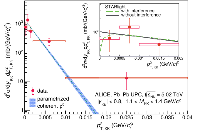
FIG. 1. Differential cross section as a function of p_{T,KK}^2 for exclusive K^+K^- photoproduction in Pb-Pb UPCs at \sqrt{s_{NN}} = 5.02 TeV and |y_{KK}| < 0.8 . The vertical lines and boxes across the data points represent statistical and systematic uncertainties, respectively. The dashed blue line and band are the result of a fit to an exponential with the fixed slope parameter b = 428 \pm 6(\text{stat}) \pm 15(\text{syst}) (GeV/ c ) ^{-2} , from a previous result on \rho^0 production [39] (see the text for details). The inset shows two curves from STARlight with and without interference between the two photon directions [14,36].
