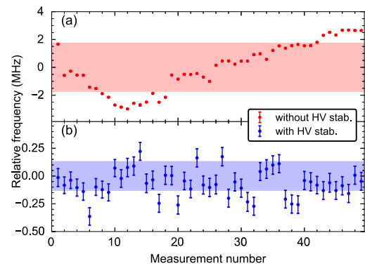
FIG. 6. Stability of the 5s^2S_{1/2} \rightarrow 5p^2P_{1/2} resonance frequency measurement in ^{88}\text{Sr}^+ with and without active high-voltage stabilization of the ions' starting potential. Particularly in the first hour after starting the power supply, the output voltage slowly settles, which was the case in (a). Due to the Doppler effect, the determined frequency changes with the starting potential and, hence, the ion velocity drift. This can be circumvented when using active high-voltage stabilization, as shown in (b), which was also measured in the first hour after starting the power supply. The shaded area corresponds to the standard deviation and decreases from 1.7 MHz to 130 kHz if the voltage-stabilization is active. The error bars in (a) and (b) depict the statistical uncertainty, which is similar for all measurements.
