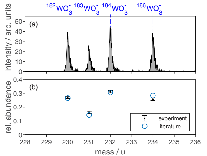
FIG. 11. (a) Spectrum of anionic signals around A = 232 from new laser-ablation spot. (b) Relative abundance of recorded signals (black) and natural abundance distribution of tungsten isotopes (blue) [68].
