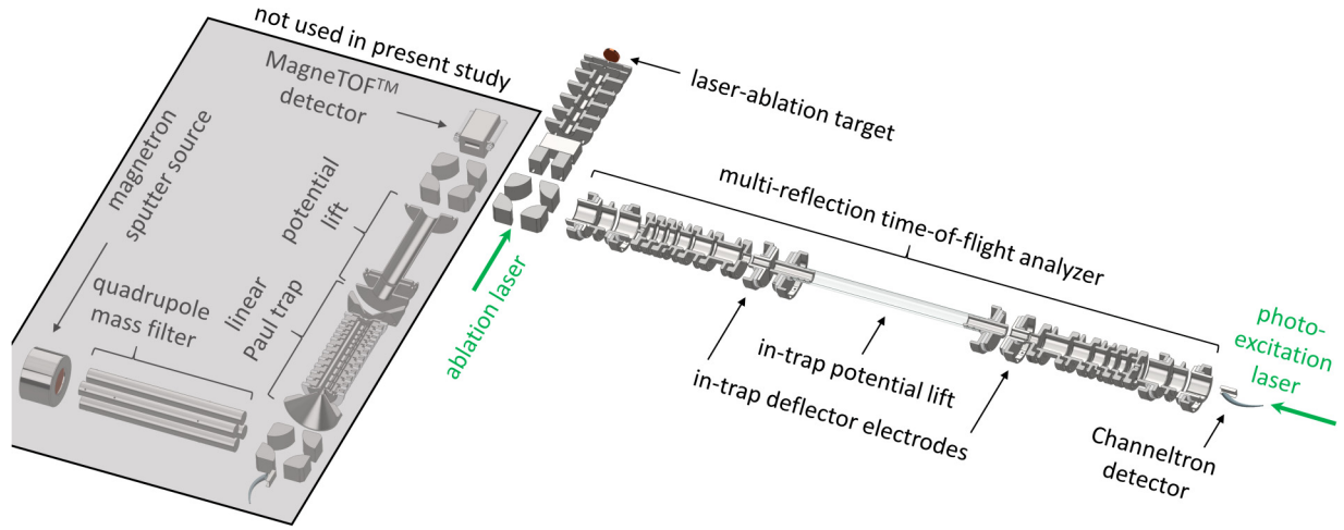
FIG. 1. Experimental setup [24] of which only the right-hand side is used in this study. The distance between components is not to scale and ion-optical components are omitted for clarity.
