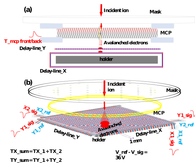
Figure 7. (a) shows the schematic cross-sectional view of the setup for the calibration of the DLD system. (b) indicates the 3D imaging principle of the calibration setup [36].
