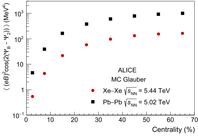
Fig. 5. The expected CME signal as a function of centrality from MC Glauber simulations for Xe-Xe and Pb-Pb collisions [73] (see text for details).
