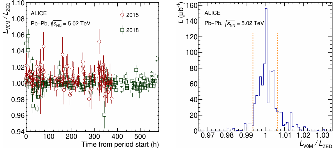
Figure 6. Left: ratio of V0M and ZED luminosities calculated according to eq. (3.5) as a function of time with respect to the beginning of the data-taking periods for 2015 (circles) and 2018 (squares). The uncertainties are statistical. Right: distribution of the ratios for all runs (2015 and 2018), weighted with the run luminosity. The dashed vertical lines are located at L_{V0M}/L_{ZED} = 1 \pm \alpha , where \alpha \sim 0.007 is the mean quadratic difference from unity.
