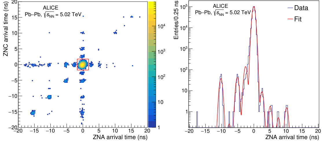
Figure 1. Left: correlation between the arrival times, relative to main–main collisions, of signals in ZNA and ZNC for events triggered by V0M. The square box depicts the satellite-collision rejection cut discussed in the text. Events outside the box are from main–satellite collisions (horizontal and vertical bands) and from satellite–satellite collisions (diagonal band). Right: distribution of the arrival time, relative to main–main collisions, in one of the two neutron calorimeters for ZED-triggered single-side neutron events. The superimposed curve shows a fit with a sum of Gaussian distributions. Both figures are for head-on collisions ( \Delta x = \Delta y = 0 ).
