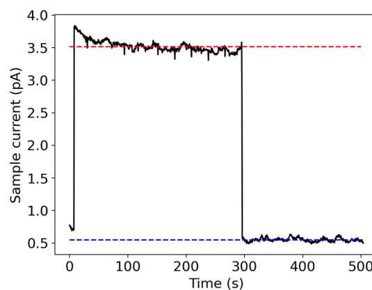
Fig. 4 Measured ion current on the sample holder during a 288 s-implantation of ^{225}\text{AcF}_2^+ from a \text{UC}_x target at 2050°C. The average ion current during implantation is indicated with a red dashed line and the average background reading without incident ion beam is indicated in blue. Values shown are after correction for secondary electron emission
