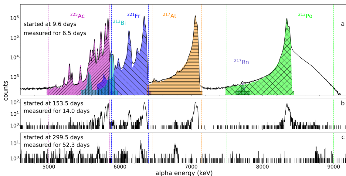
Fig. 5 \alpha decay spectrum of an ion-implanted sample collected on A/q = 263 ( ^{225}\text{AcF}_2^+ ) from a \text{UC}_x target at 2067(50)^\circ\text{C} with a gas mix of 40% \text{CF}_4 , 60% \text{Ar} (see also Table 1). The spectra start times and measurement lengths are indicated on the left. Characteristic \alpha decays
