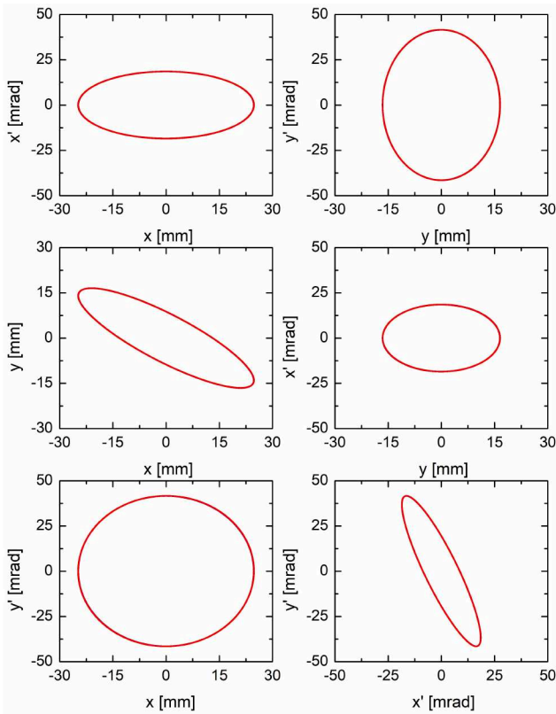
Figure 2: From full 4D-periodic solution: projected 4\times\text{rms} ellipses of the beam second moments matrix at the entrance (blue) and exit (red) of the periodic channel for a coupled proton beam with 10 mA. It is obtained that C^6(s_2) \approx C^6(s_2 + \ell) .
