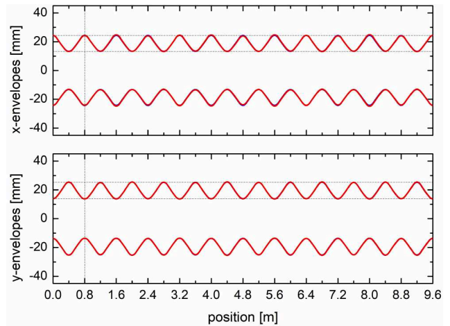
Figure 4: From full 4D-periodic solution: horizontal and vertical 2\times\text{rms} -beam sizes of a coupled 10 mA proton beam along a regular FODO quadrupole channel as obtained from rms tracking (blue) and particle tracking (red). The initial particle distribution is rms equivalent to matrix C^6(s_2) .
