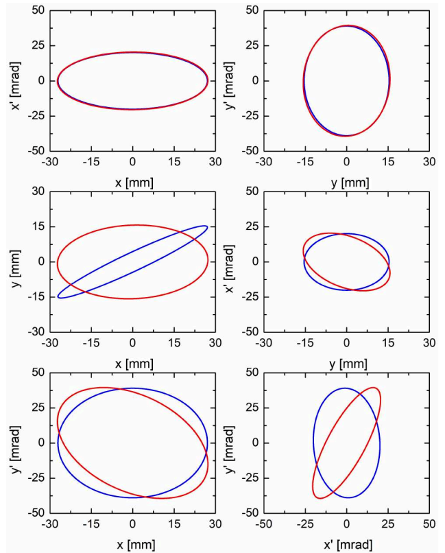
Figure 3: From simple 2D-envelope matching: projected 4\times\text{rms} ellipses of the beam second moments matrix at the entrance (blue) and exit (red) of the periodic channel for a coupled proton beam with 10 mA. It is obtained that C^\dagger(s_2) \neq C^\dagger(s_2 + \ell) .
