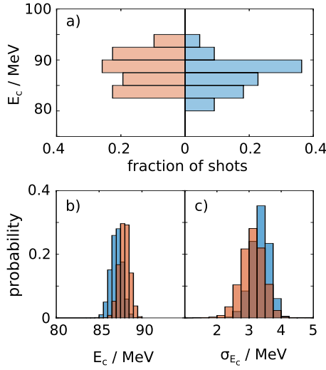
Fig. 4. a) Distribution of inferred value for the \gamma photon spectrum E_c for 32 null shots (blue) and 22 collision shots (red) b) Bootstrap estimate of the mean of E_c for null shots (blue) and collision shots (red) c) Bootstrap estimate of the standard deviation of E_c for null shots (blue) and collision shots (red).
