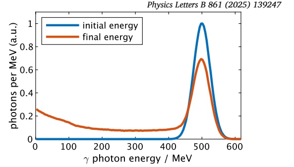
Fig. 1. Illustration of the effect on the photon energy spectrum of copious photon-photon scattering of a 500 \pm 25 \text{ MeV} \gamma photon beam in a very dense field of 5 \text{ keV} photons with n_x = 10^{27} \text{ photons mm}^{-3} and length 1 \text{ cm} . Scattering in such a high density field results in a broadening and downshift of the \gamma photon energy.
